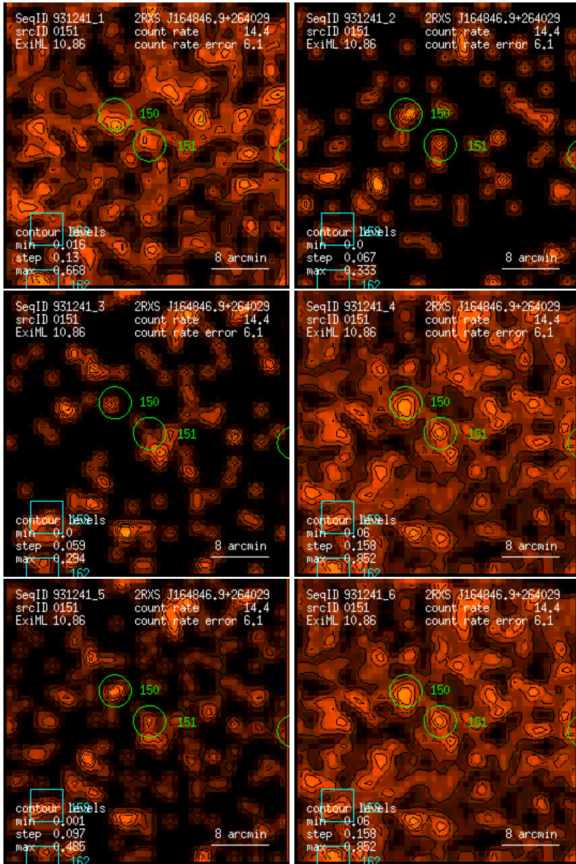
Figure 151: RASS 931241: detection 0151: band rate images, Gaussian filter: (1) PSPC channels 11 – 41, (2) 52 – 90, (3) 91 – 201, (4) 11 – 235, (5) 52 – 201, (6) 11 – 201. Broad band rates in counts/ks. Band rate contour levels in counts/ks/arcmin 2 .
