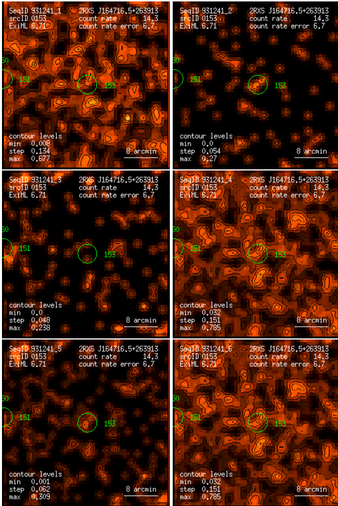
Figure 153: RASS 931241: detection 0153: band rate images, Gaussian filter: (1) PSPC channels 11 – 41, (2) 52 – 90, (3) 91 – 201, (4) 11 – 235, (5) 52 – 201, (6) 11 – 201. Broad band rates in counts/ks. Band rate contour levels in counts/ks/arcmin 2 .
