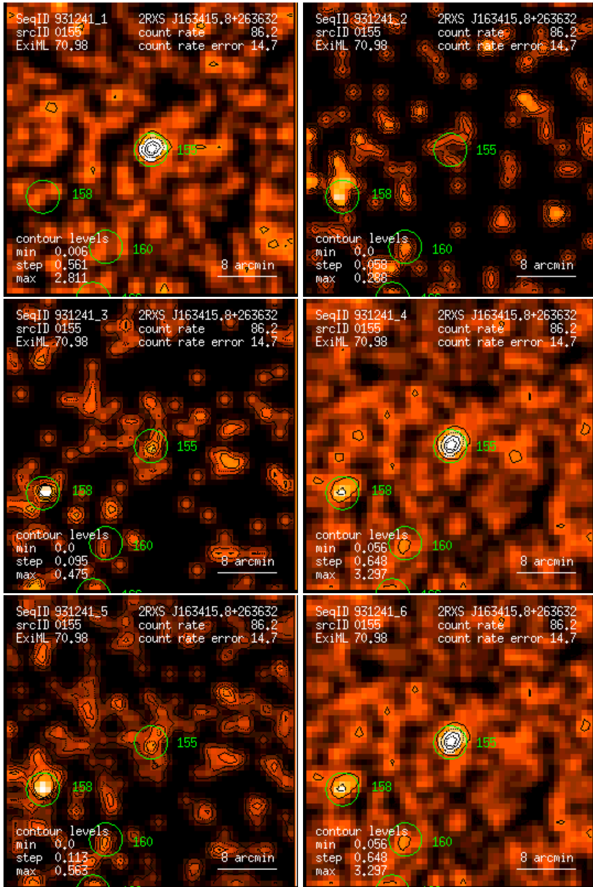
Figure 155: RASS 931241: detection 0155: band rate images, Gaussian filter: (1) PSPC channels 11 – 41, (2) 52 – 90, (3) 91 – 201, (4) 11 – 235, (5) 52 – 201, (6) 11 – 201. Broad band rates in counts/ks. Band rate contour levels in counts/ks/arcmin 2 .
