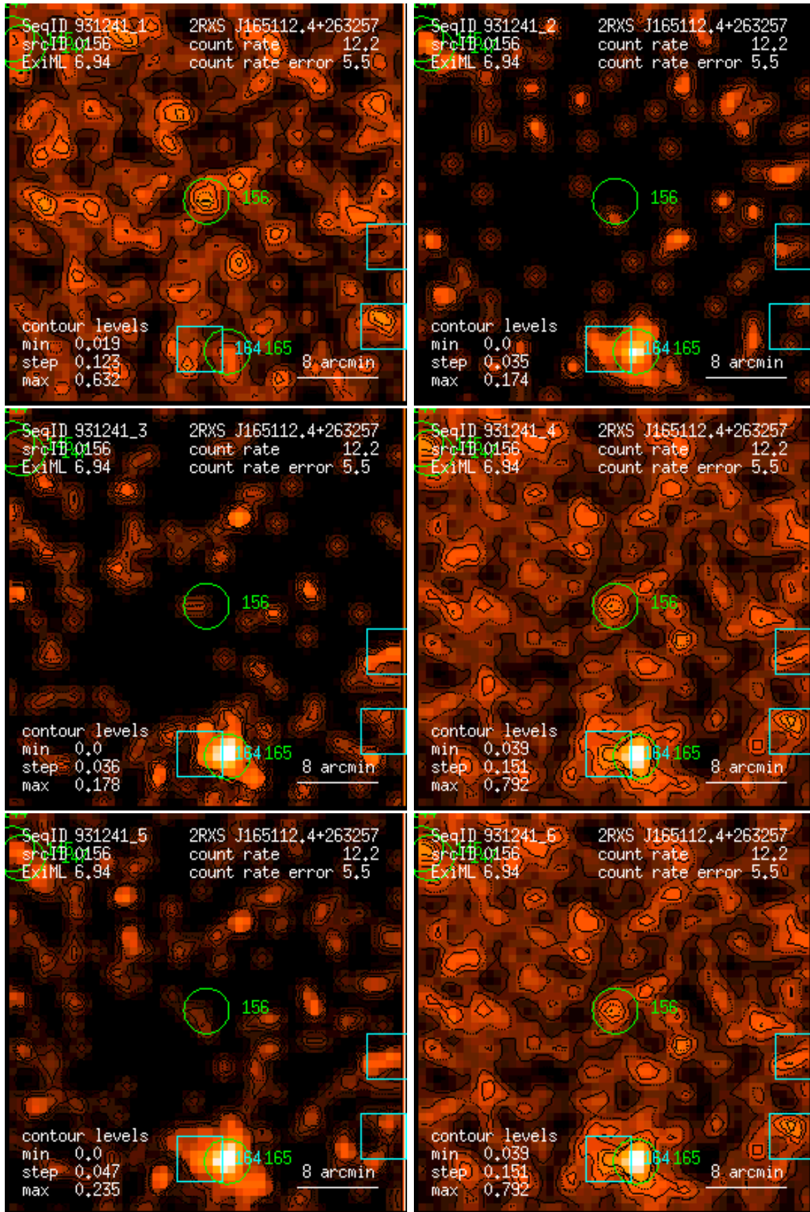
Figure 156: RASS 931241: detection 0156: band rate images, Gaussian filter: (1) PSPC channels 11 – 41, (2) 52 – 90, (3) 91 – 201, (4) 11 – 235, (5) 52 – 201, (6) 11 – 201. Broad band rates in counts/ks. Band rate contour levels in counts/ks/arcmin 2 .
