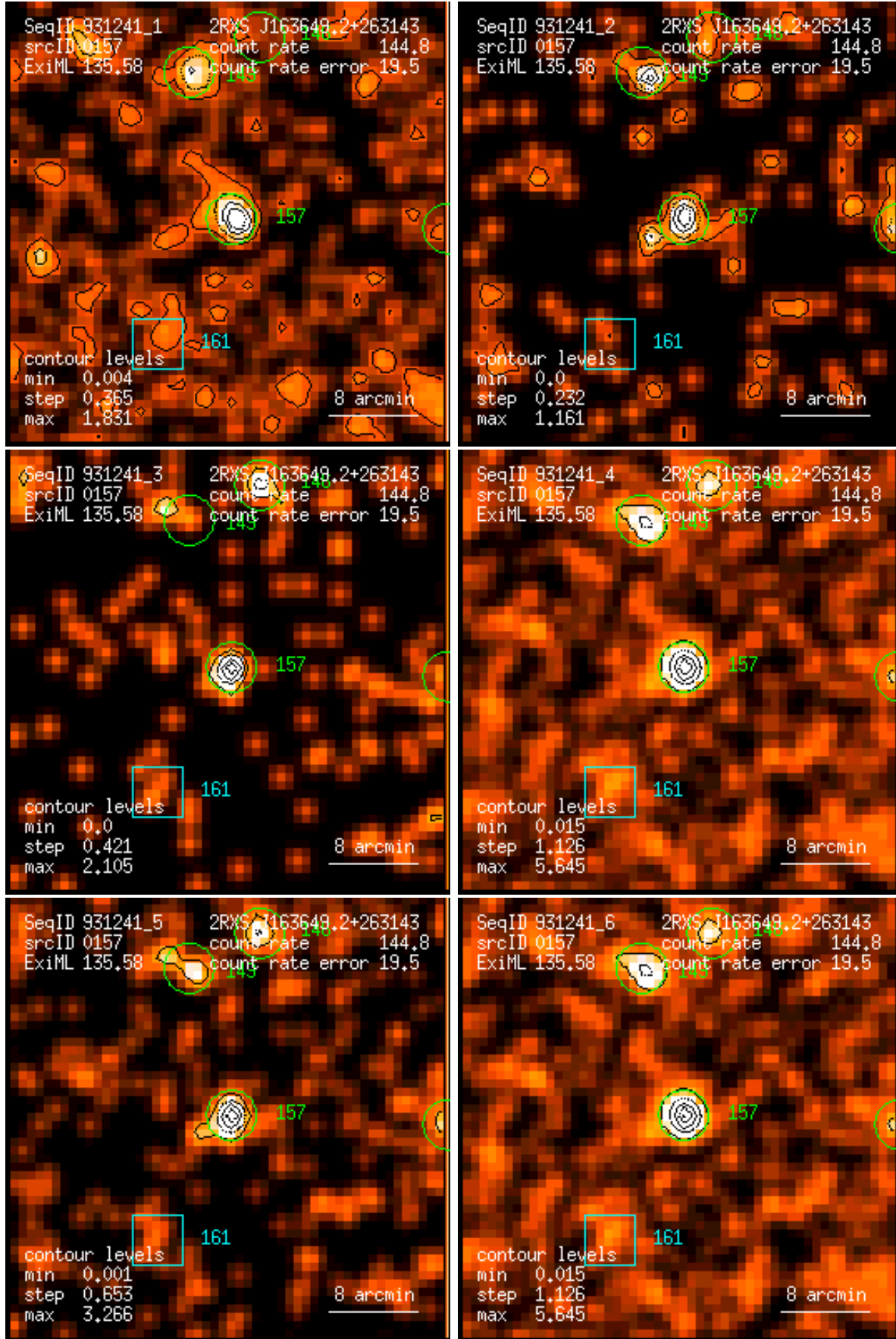
Figure 157: RASS 931241: detection 0157: band rate images, Gaussian filter: (1) PSPC channels 11 – 41, (2) 52 – 90, (3) 91 – 201, (4) 11 – 235, (5) 52 – 201, (6) 11 – 201. Broad band rates in counts/ks. Band rate contour levels in counts/ks/arcmin 2 .
