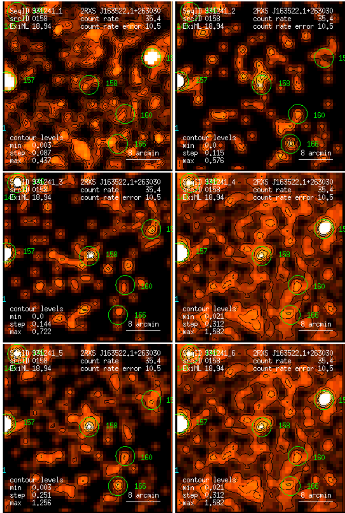
Figure 158: RASS 931241: detection 0158: band rate images, Gaussian filter: (1) PSPC channels 11 – 41, (2) 52 – 90, (3) 91 – 201, (4) 11 – 235, (5) 52 – 201, (6) 11 – 201. Broad band rates in counts/ks. Band rate contour levels in counts/ks/arcmin 2 .
