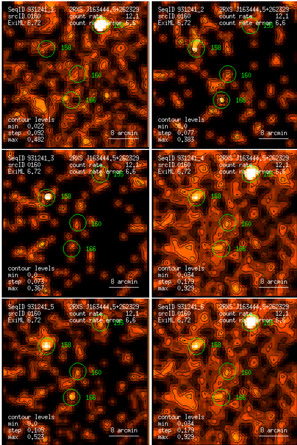
Figure 160: RASS 931241: detection 0160: band rate images, Gaussian filter: (1) PSPC channels 11 – 41, (2) 52 – 90, (3) 91 – 201, (4) 11 – 235, (5) 52 – 201, (6) 11 – 201. Broad band rates in counts/ks. Band rate contour levels in counts/ks/arcmin 2 .
