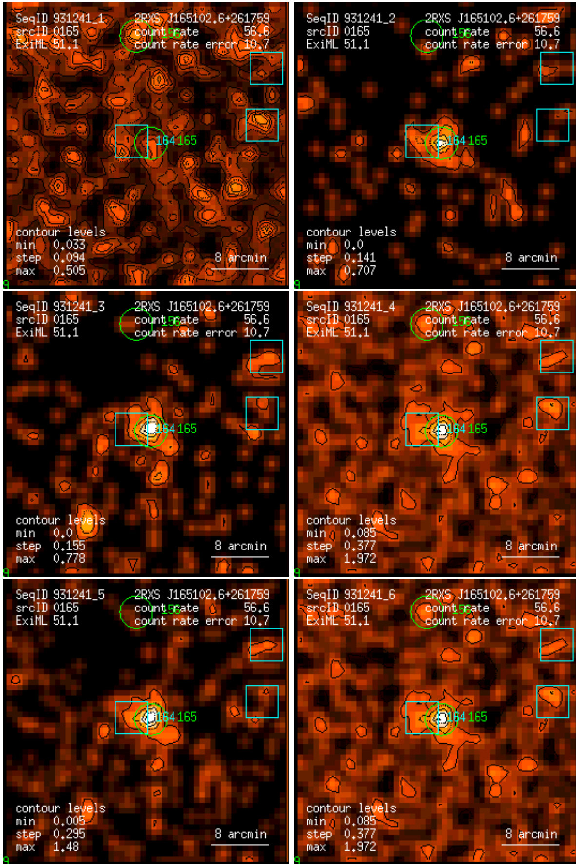
Figure 165: RASS 931241: detection 0165: band rate images, Gaussian filter: (1) PSPC channels 11 – 41, (2) 52 – 90, (3) 91 – 201, (4) 11 – 235, (5) 52 – 201, (6) 11 – 201. Broad band rates in counts/ks. Band rate contour levels in counts/ks/arcmin 2 .
