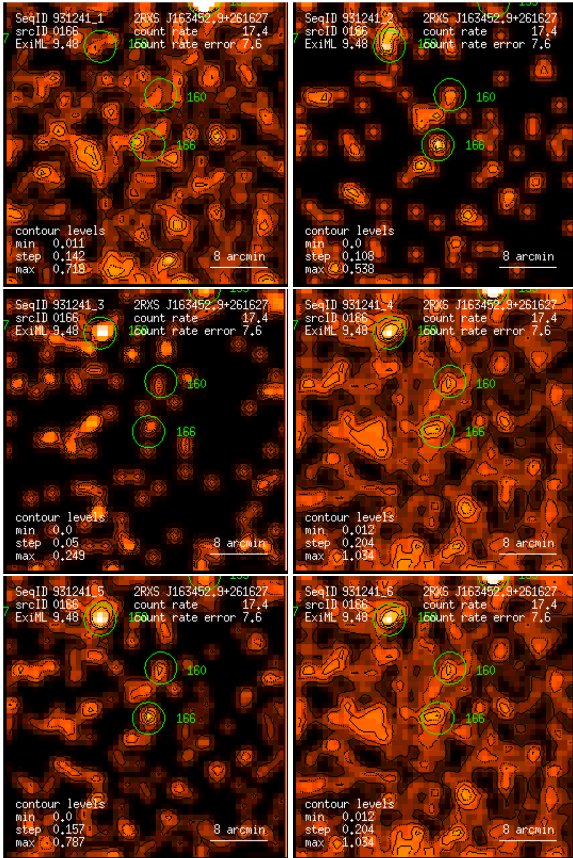
Figure 166: RASS 931241: detection 0166: band rate images, Gaussian filter: (1) PSPC channels 11 – 41, (2) 52 – 90, (3) 91 – 201, (4) 11 – 235, (5) 52 – 201, (6) 11 – 201. Broad band rates in counts/ks. Band rate contour levels in counts/ks/arcmin 2 .
