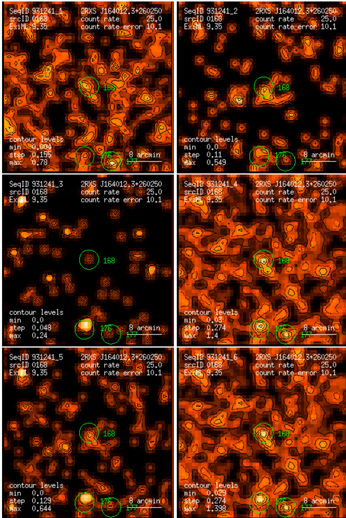
Figure 168: RASS 931241: detection 0168: band rate images, Gaussian filter: (1) PSPC channels 11 – 41, (2) 52 – 90, (3) 91 – 201, (4) 11 – 235, (5) 52 – 201, (6) 11 – 201. Broad band rates in counts/ks. Band rate contour levels in counts/ks/arcmin 2 .
