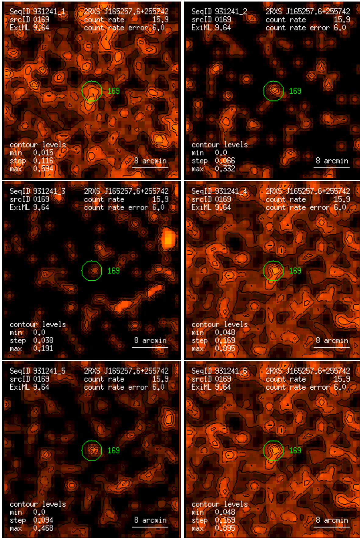
Figure 169: RASS 931241: detection 0169: band rate images, Gaussian filter: (1) PSPC channels 11 – 41, (2) 52 – 90, (3) 91 – 201, (4) 11 – 235, (5) 52 – 201, (6) 11 – 201. Broad band rates in counts/ks. Band rate contour levels in counts/ks/arcmin 2 .
