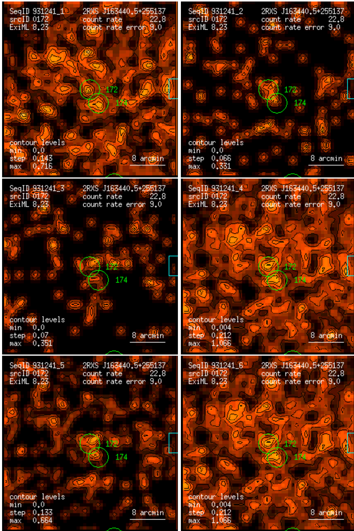
Figure 172: RASS 931241: detection 0172: band rate images, Gaussian filter: (1) PSPC channels 11 – 41, (2) 52 – 90, (3) 91 – 201, (4) 11 – 235, (5) 52 – 201, (6) 11 – 201. Broad band rates in counts/ks. Band rate contour levels in counts/ks/arcmin 2 .
