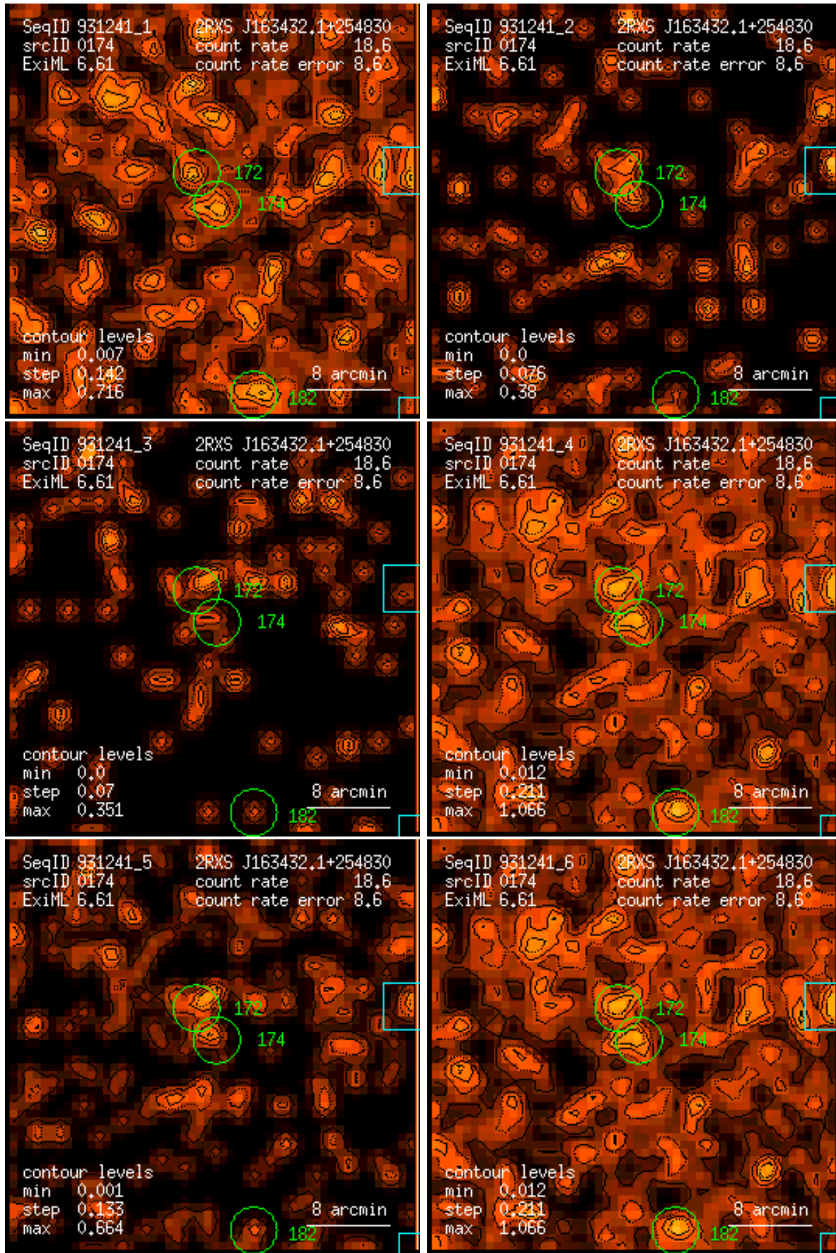
Figure 174: RASS 931241: detection 0174: band rate images, Gaussian filter: (1) PSPC channels 11 – 41, (2) 52 – 90, (3) 91 – 201, (4) 11 – 235, (5) 52 – 201, (6) 11 – 201. Broad band rates in counts/ks. Band rate contour levels in counts/ks/arcmin 2 .
