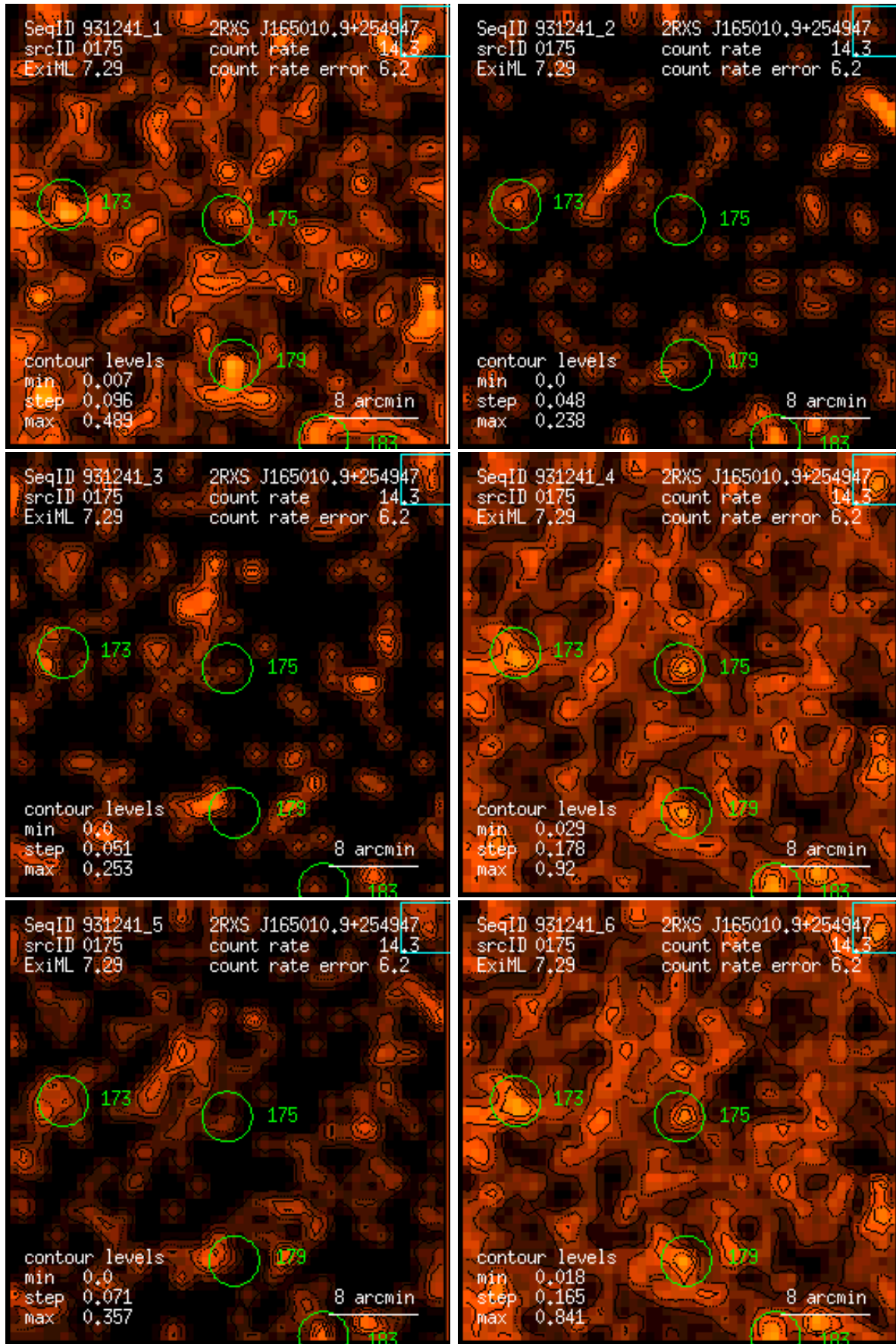
Figure 175: RASS 931241: detection 0175: band rate images, Gaussian filter: (1) PSPC channels 11 – 41, (2) 52 – 90, (3) 91 – 201, (4) 11 – 235, (5) 52 – 201, (6) 11 – 201. Broad band rates in counts/ks. Band rate contour levels in counts/ks/arcmin 2 .
