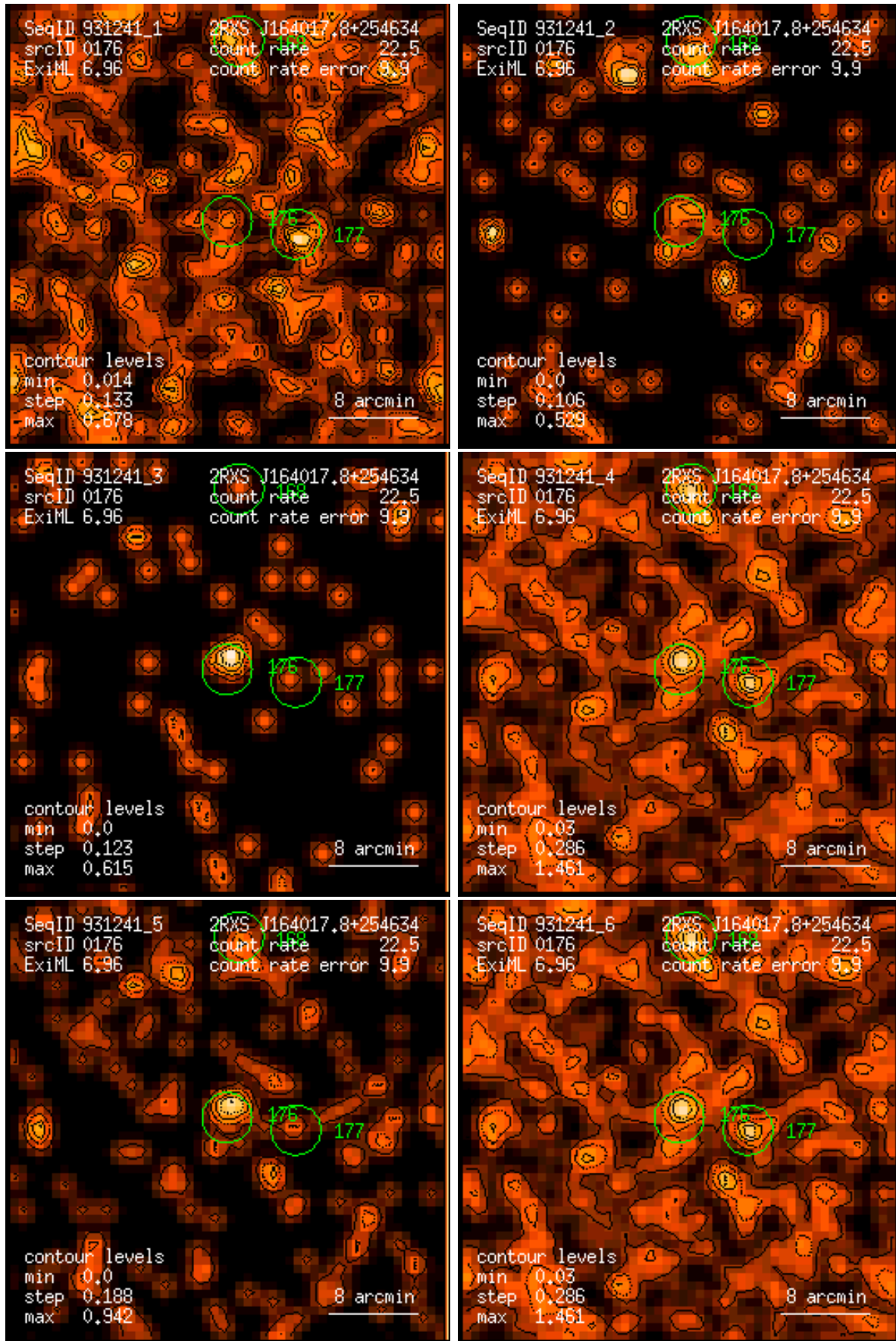
Figure 176: RASS 931241: detection 0176: band rate images, Gaussian filter: (1) PSPC channels 11 – 41, (2) 52 – 90, (3) 91 – 201, (4) 11 – 235, (5) 52 – 201, (6) 11 – 201. Broad band rates in counts/ks. Band rate contour levels in counts/ks/arcmin 2 .
