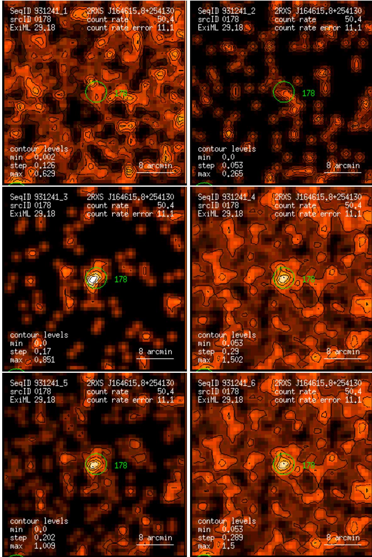
Figure 178: RASS 931241: detection 0178: band rate images, Gaussian filter: (1) PSPC channels 11 – 41, (2) 52 – 90, (3) 91 – 201, (4) 11 – 235, (5) 52 – 201, (6) 11 – 201. Broad band rates in counts/ks. Band rate contour levels in counts/ks/arcmin 2 .
