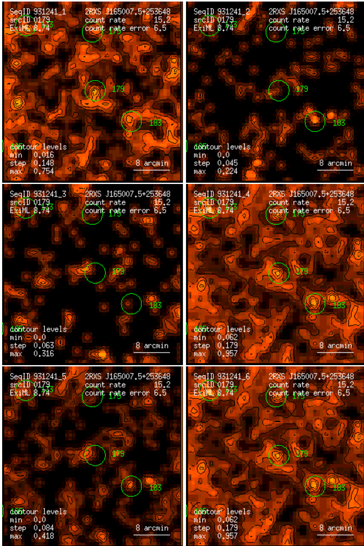
Figure 179: RASS 931241: detection 0179: band rate images, Gaussian filter: (1) PSPC channels 11 – 41, (2) 52 – 90, (3) 91 – 201, (4) 11 – 235, (5) 52 – 201, (6) 11 – 201. Broad band rates in counts/ks. Band rate contour levels in counts/ks/arcmin 2 .
