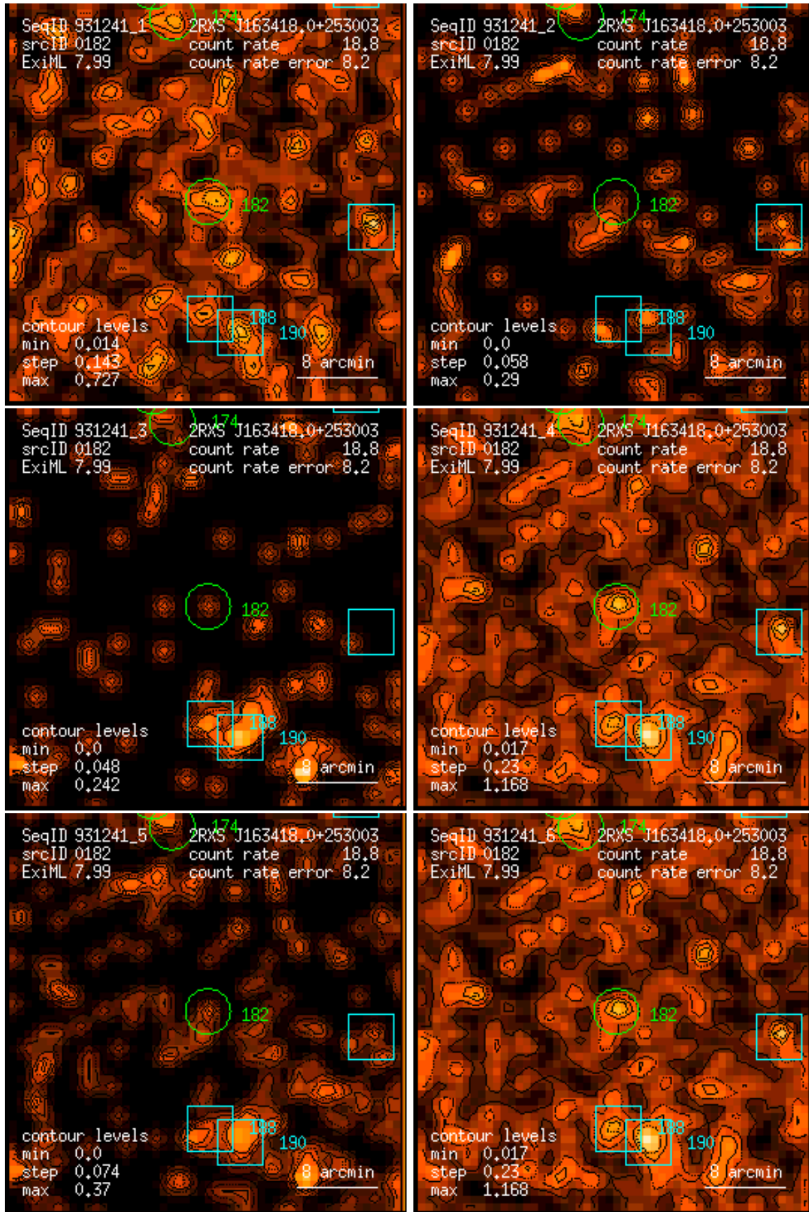
Figure 182: RASS 931241: detection 0182: band rate images, Gaussian filter: (1) PSPC channels 11 – 41, (2) 52 – 90, (3) 91 – 201, (4) 11 – 235, (5) 52 – 201, (6) 11 – 201. Broad band rates in counts/ks. Band rate contour levels in counts/ks/arcmin 2 .
