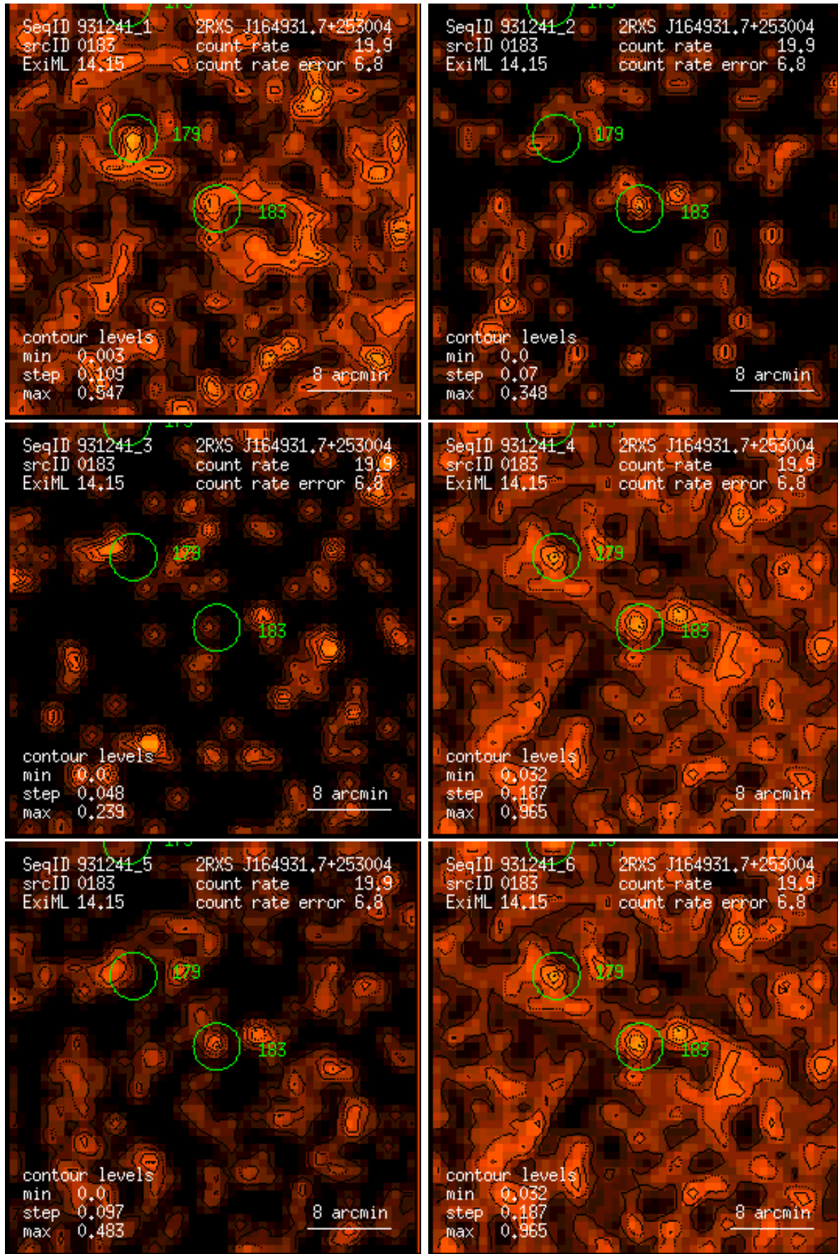
Figure 183: RASS 931241: detection 0183: band rate images, Gaussian filter: (1) PSPC channels 11 – 41, (2) 52 – 90, (3) 91 – 201, (4) 11 – 235, (5) 52 – 201, (6) 11 – 201. Broad band rates in counts/ks. Band rate contour levels in counts/ks/arcmin 2 .
