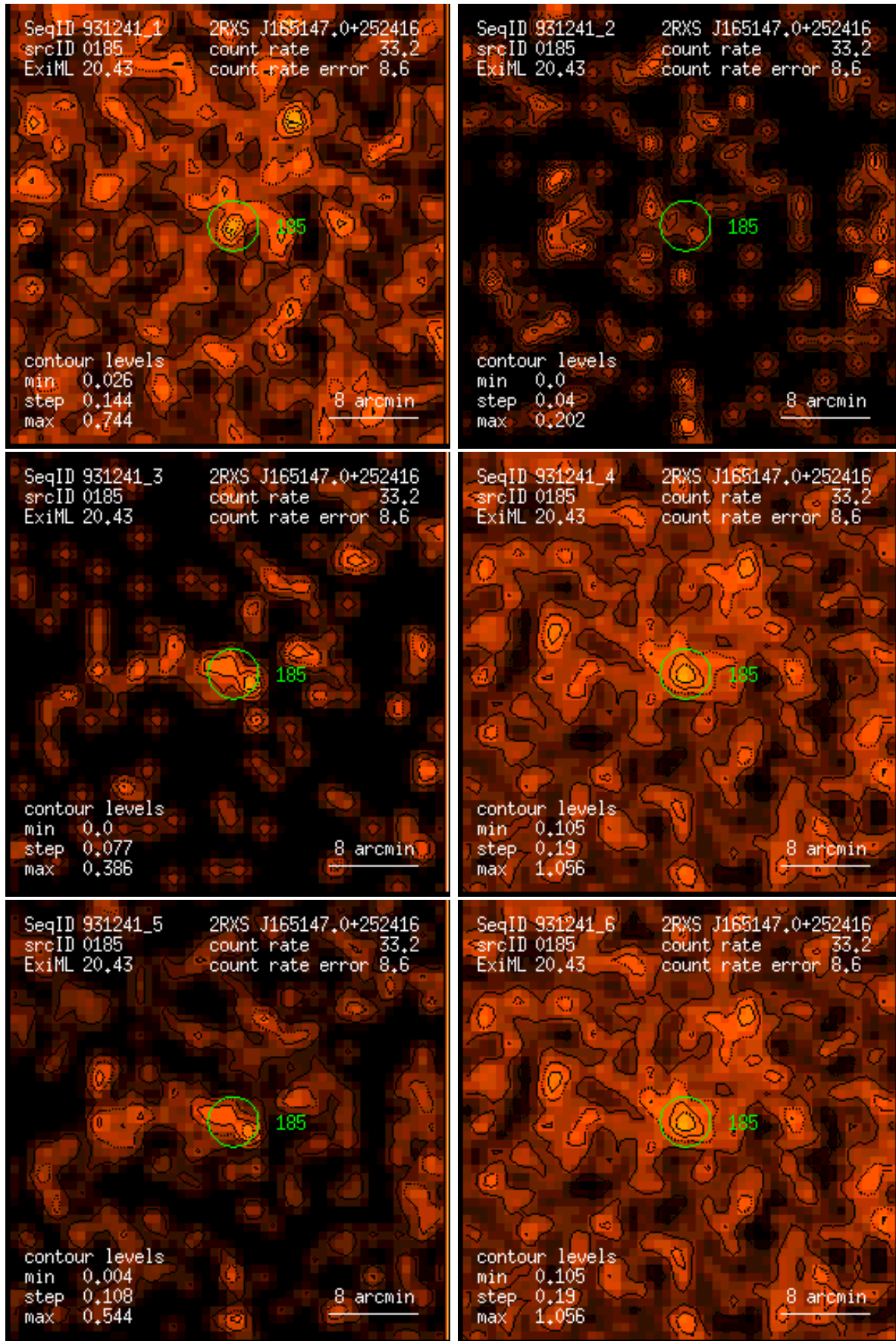
Figure 185: RASS 931241: detection 0185: band rate images, Gaussian filter: (1) PSPC channels 11 – 41, (2) 52 – 90, (3) 91 – 201, (4) 11 – 235, (5) 52 – 201, (6) 11 – 201. Broad band rates in counts/ks. Band rate contour levels in counts/ks/arcmin 2 .
