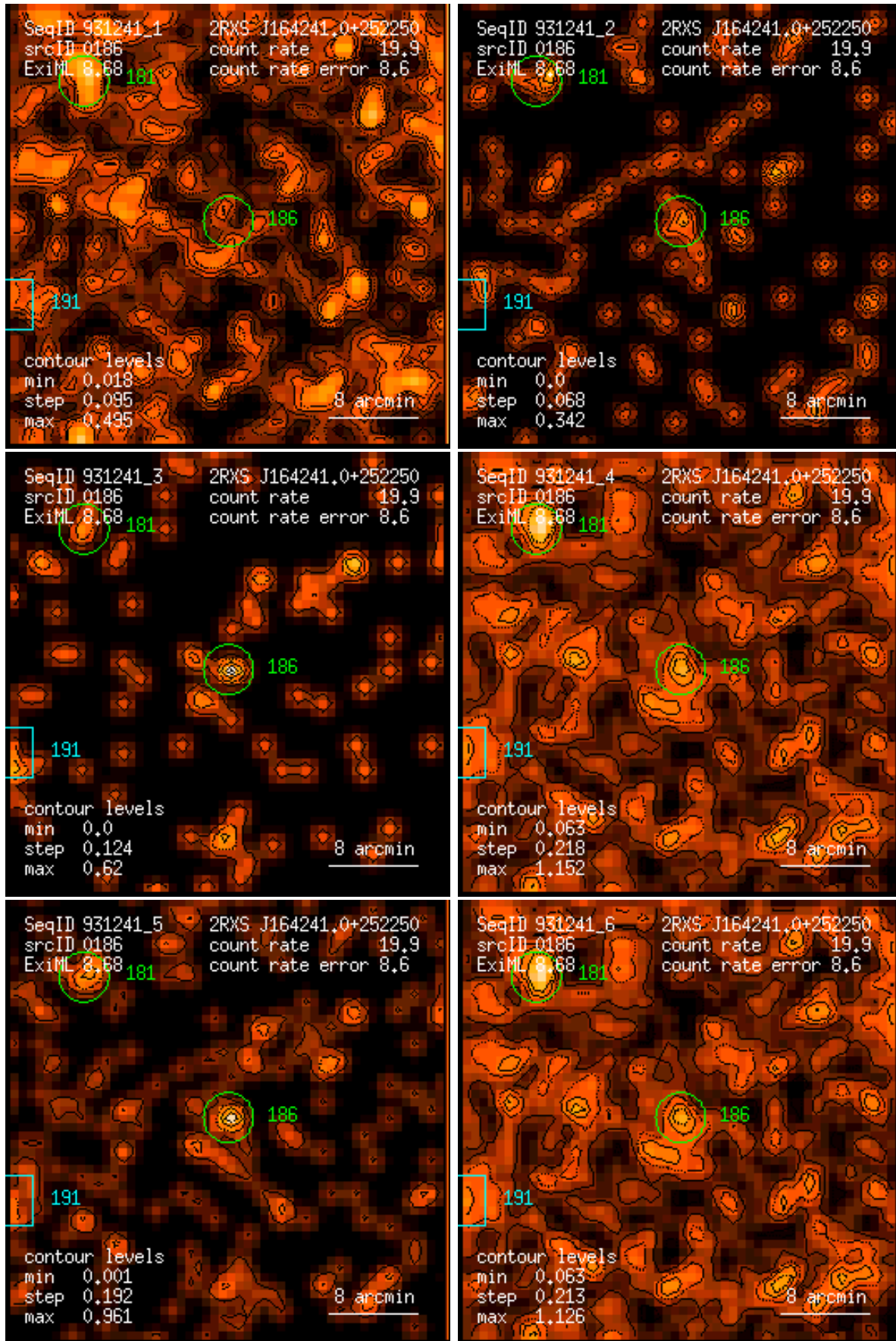
Figure 186: RASS 931241: detection 0186: band rate images, Gaussian filter: (1) PSPC channels 11 – 41, (2) 52 – 90, (3) 91 – 201, (4) 11 – 235, (5) 52 – 201, (6) 11 – 201. Broad band rates in counts/ks. Band rate contour levels in counts/ks/arcmin 2 .
