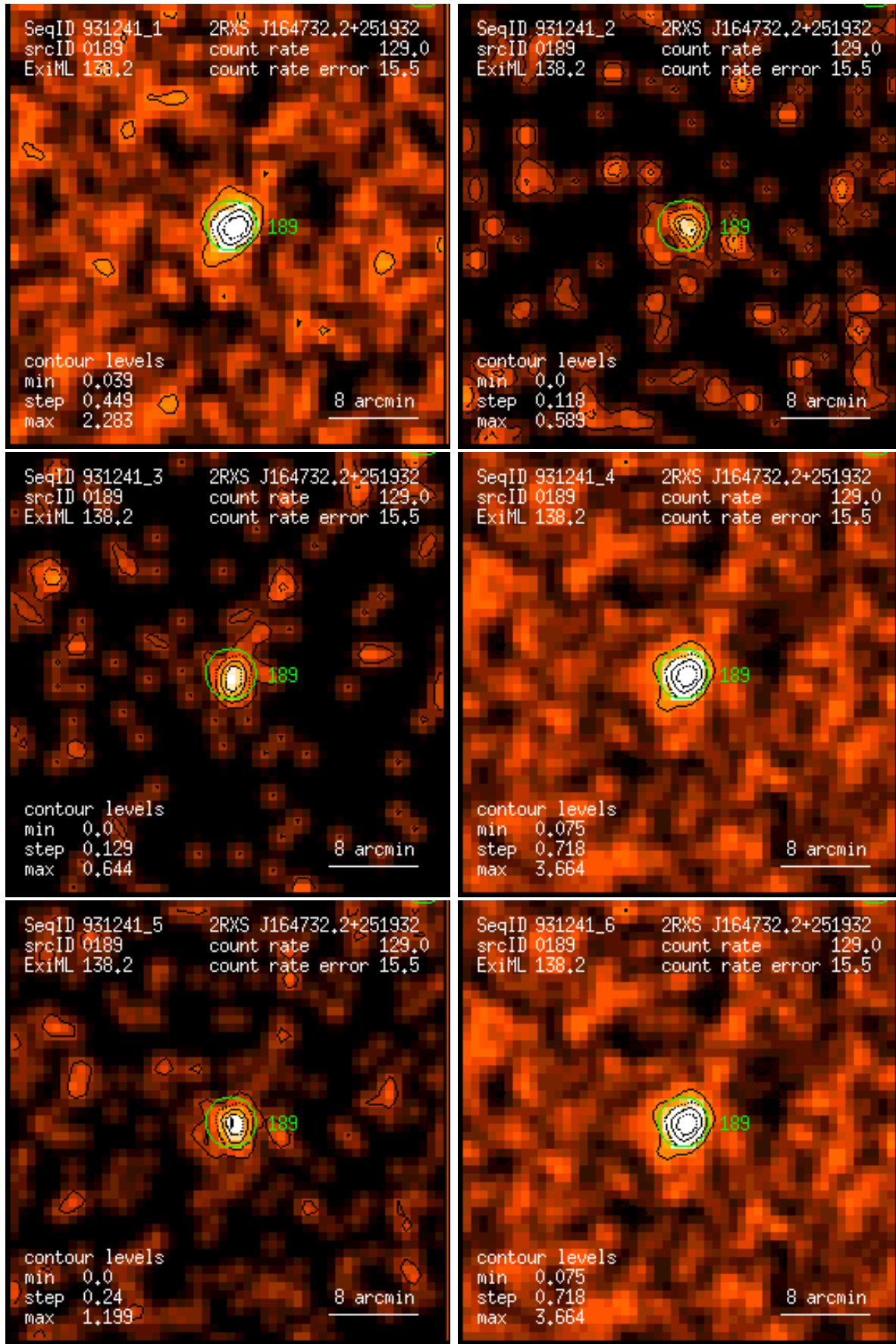
Figure 189: RASS 931241: detection 0189: band rate images, Gaussian filter: (1) PSPC channels 11 – 41, (2) 52 – 90, (3) 91 – 201, (4) 11 – 235, (5) 52 – 201, (6) 11 – 201. Broad band rates in counts/ks. Band rate contour levels in counts/ks/arcmin 2 .
