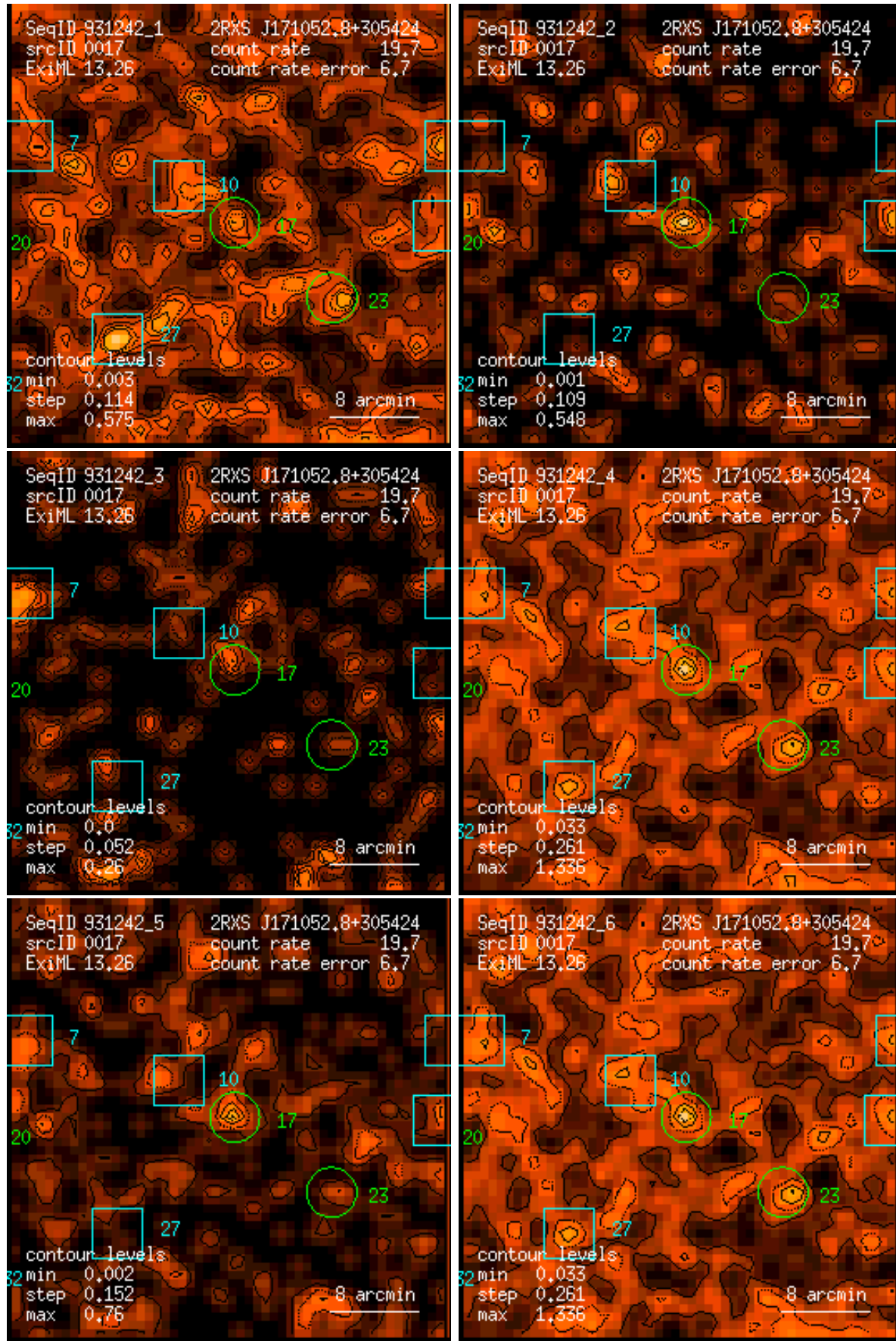
Figure 17: RASS 931242: detection 0017: band rate images, Gaussian filter: (1) PSPC channels 11 – 41, (2) 52 – 90, (3) 91 – 201, (4) 11 – 235, (5) 52 – 201, (6) 11 – 201. Broad band rates in counts/ks. Band rate contour levels in counts/ks/arcmin 2 .
