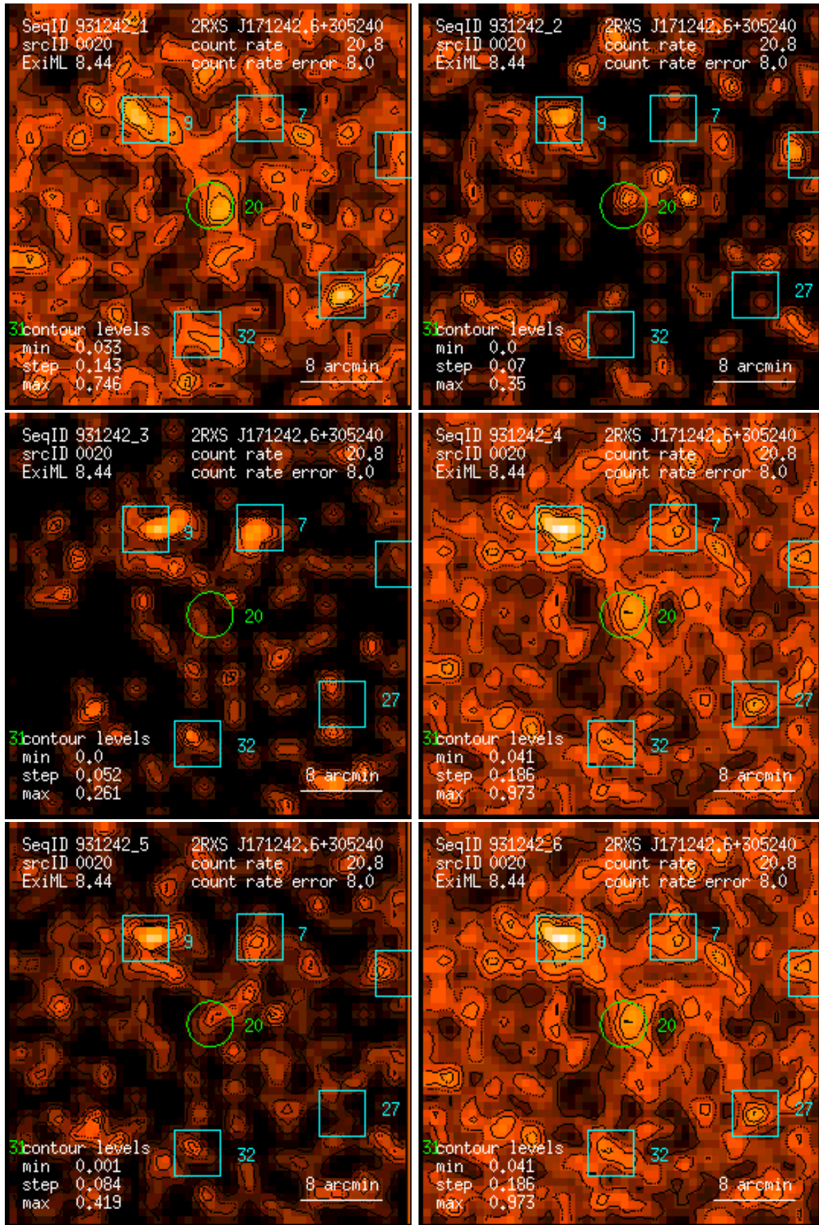
Figure 20: RASS 931242: detection 0020: band rate images, Gaussian filter: (1) PSPC channels 11 – 41, (2) 52 – 90, (3) 91 – 201, (4) 11 – 235, (5) 52 – 201, (6) 11 – 201. Broad band rates in counts/ks. Band rate contour levels in counts/ks/arcmin 2 .
