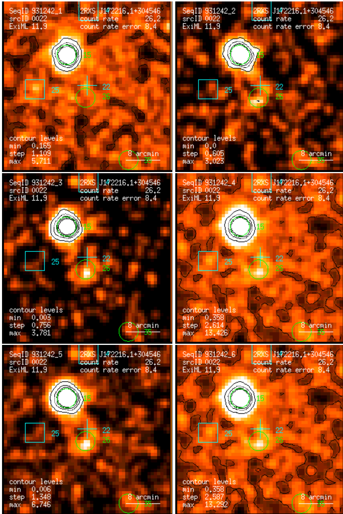
Figure 22: RASS 931242: detection 0022: band rate images, Gaussian filter: (1) PSPC channels 11 – 41, (2) 52 – 90, (3) 91 – 201, (4) 11 – 235, (5) 52 – 201, (6) 11 – 201. Broad band rates in counts/ks. Band rate contour levels in counts/ks/arcmin 2 .
