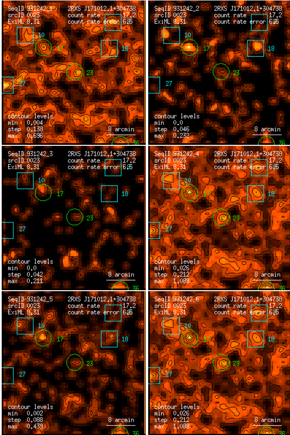
Figure 23: RASS 931242: detection 0023: band rate images, Gaussian filter: (1) PSPC channels 11 – 41, (2) 52 – 90, (3) 91 – 201, (4) 11 – 235, (5) 52 – 201, (6) 11 – 201. Broad band rates in counts/ks. Band rate contour levels in counts/ks/arcmin 2 .
