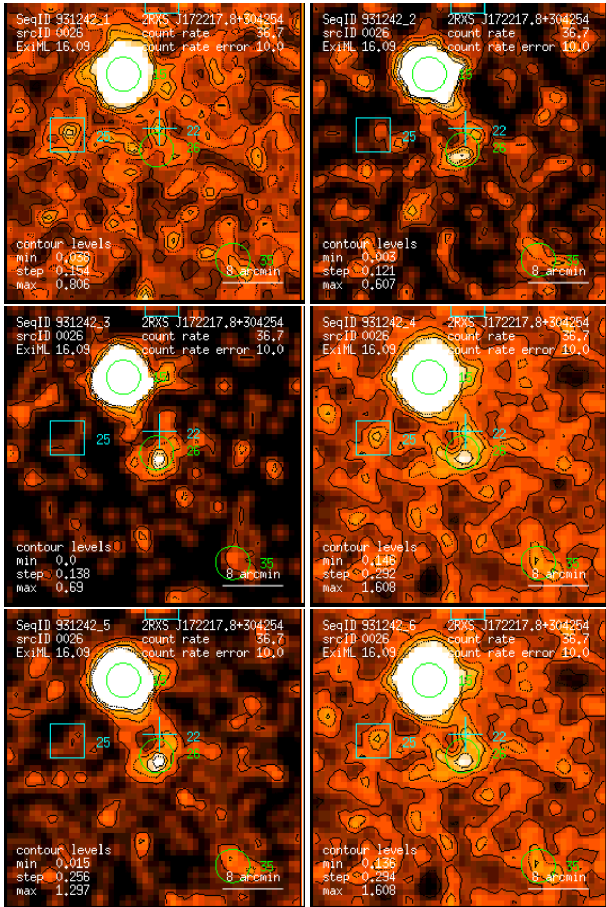
Figure 26: RASS 931242: detection 0026: band rate images, Gaussian filter: (1) PSPC channels 11 – 41, (2) 52 – 90, (3) 91 – 201, (4) 11 – 235, (5) 52 – 201, (6) 11 – 201. Broad band rates in counts/ks. Band rate contour levels in counts/ks/arcmin 2 .
