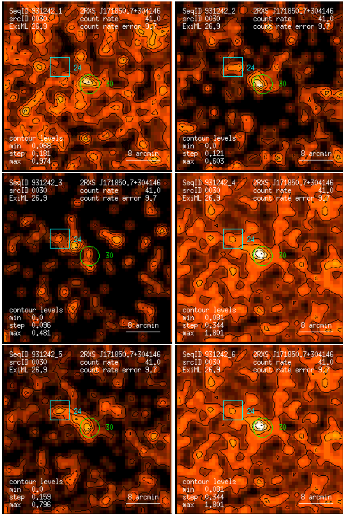
Figure 30: RASS 931242: detection 0030: band rate images, Gaussian filter: (1) PSPC channels 11 – 41, (2) 52 – 90, (3) 91 – 201, (4) 11 – 235, (5) 52 – 201, (6) 11 – 201. Broad band rates in counts/ks. Band rate contour levels in counts/ks/arcmin 2 .
