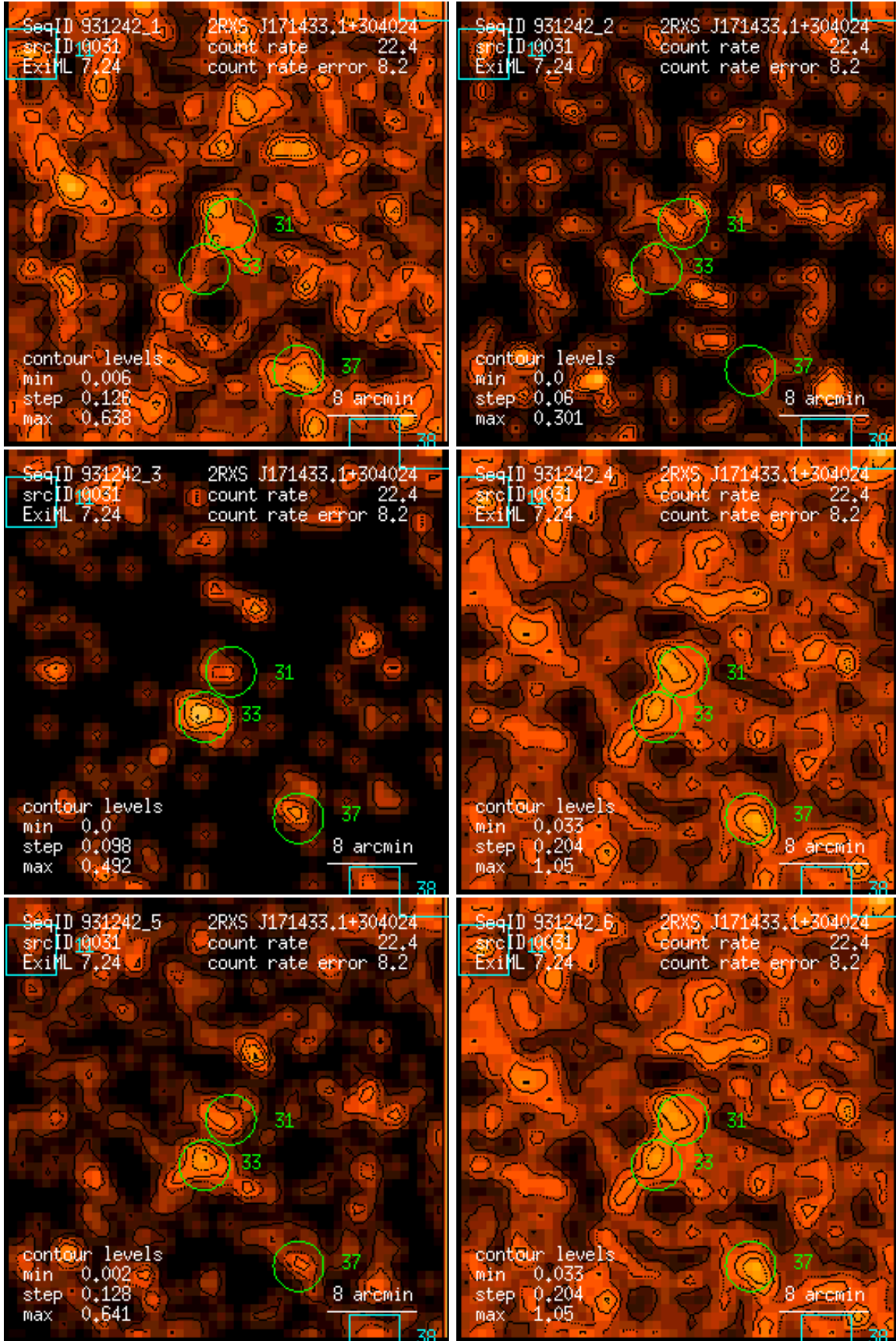
Figure 31: RASS 931242: detection 0031: band rate images, Gaussian filter: (1) PSPC channels 11 – 41, (2) 52 – 90, (3) 91 – 201, (4) 11 – 235, (5) 52 – 201, (6) 11 – 201. Broad band rates in counts/ks. Band rate contour levels in counts/ks/arcmin 2 .
