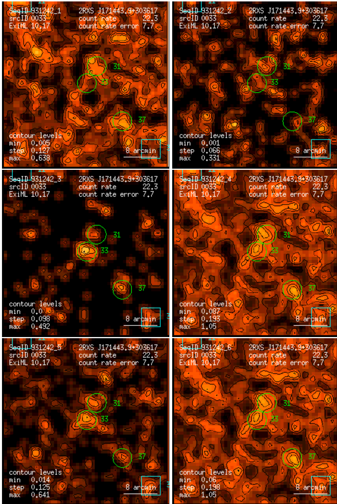
Figure 33: RASS 931242: detection 0033: band rate images, Gaussian filter: (1) PSPC channels 11 – 41, (2) 52 – 90, (3) 91 – 201, (4) 11 – 235, (5) 52 – 201, (6) 11 – 201. Broad band rates in counts/ks. Band rate contour levels in counts/ks/arcmin 2 .
