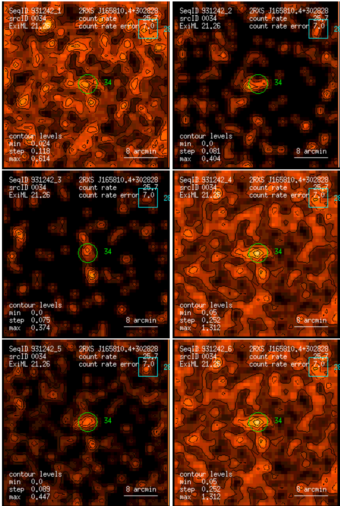
Figure 34: RASS 931242: detection 0034: band rate images, Gaussian filter: (1) PSPC channels 11 – 41, (2) 52 – 90, (3) 91 – 201, (4) 11 – 235, (5) 52 – 201, (6) 11 – 201. Broad band rates in counts/ks. Band rate contour levels in counts/ks/arcmin 2 .
