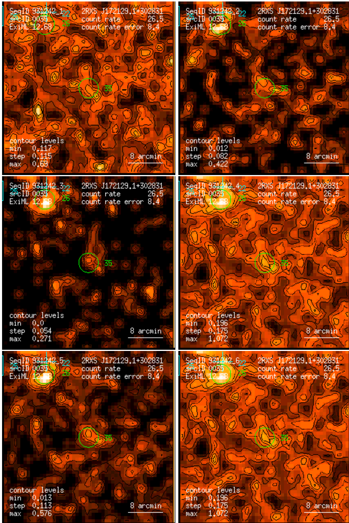
Figure 35: RASS 931242: detection 0035: band rate images, Gaussian filter: (1) PSPC channels 11 – 41, (2) 52 – 90, (3) 91 – 201, (4) 11 – 235, (5) 52 – 201, (6) 11 – 201. Broad band rates in counts/ks. Band rate contour levels in counts/ks/arcmin 2 .
