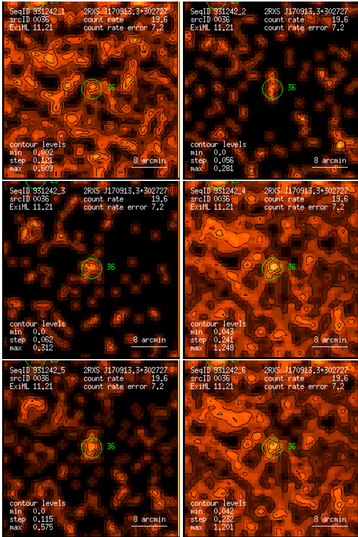
Figure 36: RASS 931242: detection 0036: band rate images, Gaussian filter: (1) PSPC channels 11 – 41, (2) 52 – 90, (3) 91 – 201, (4) 11 – 235, (5) 52 – 201, (6) 11 – 201. Broad band rates in counts/ks. Band rate contour levels in counts/ks/arcmin 2 .
