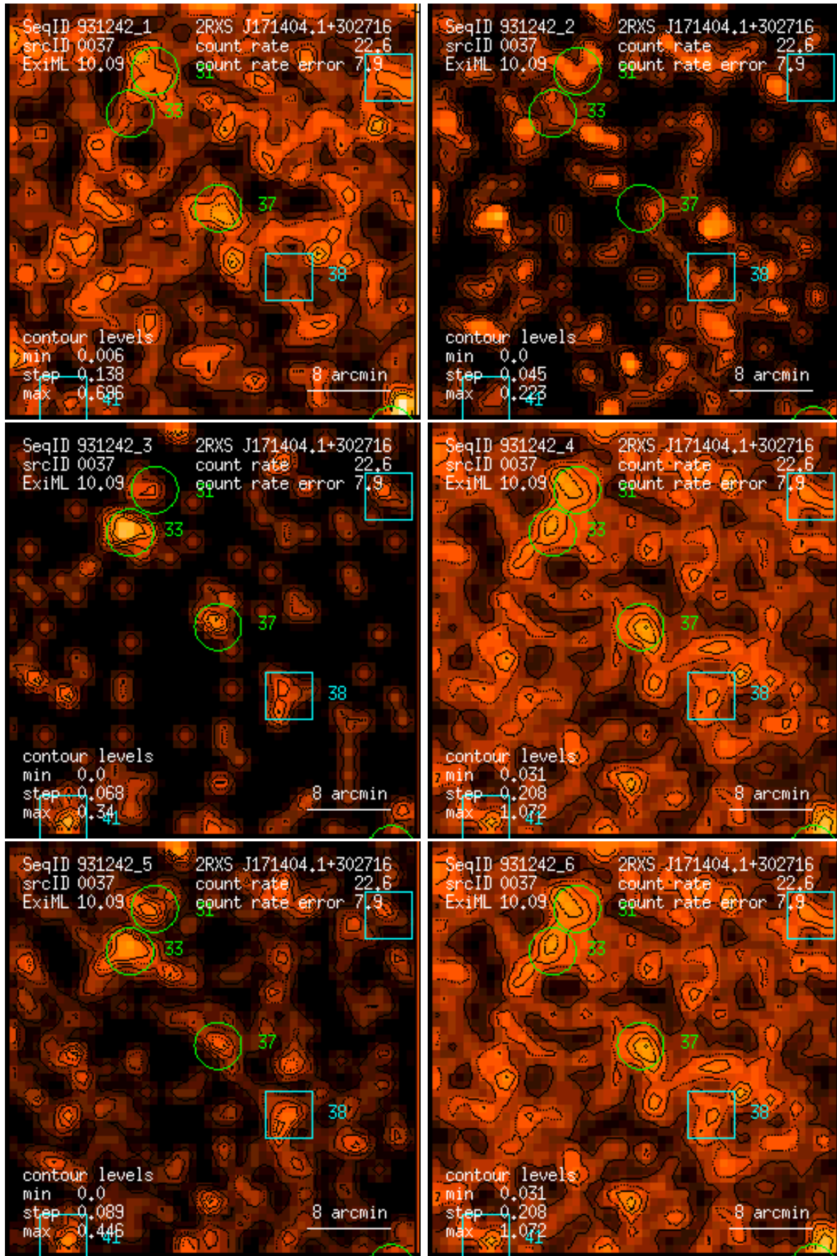
Figure 37: RASS 931242: detection 0037: band rate images, Gaussian filter: (1) PSPC channels 11 – 41, (2) 52 – 90, (3) 91 – 201, (4) 11 – 235, (5) 52 – 201, (6) 11 – 201. Broad band rates in counts/ks. Band rate contour levels in counts/ks/arcmin 2 .
