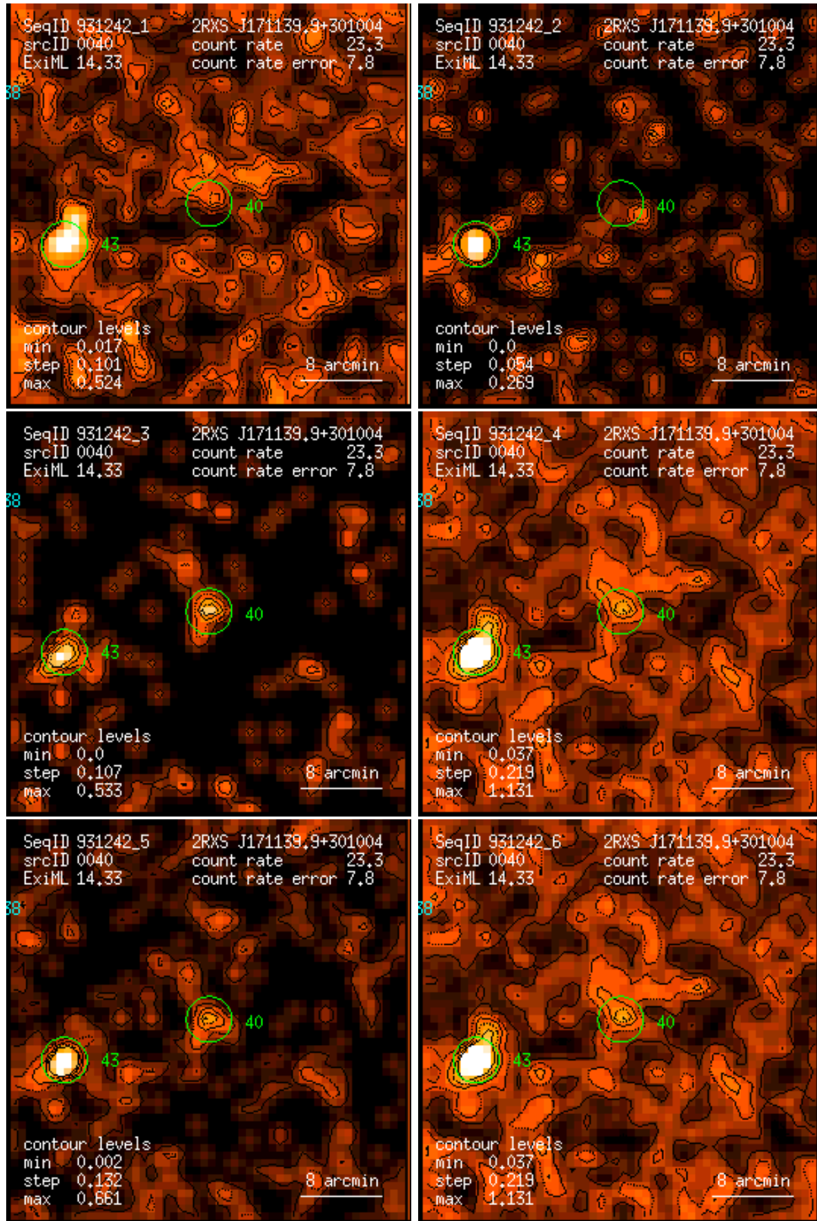
Figure 40: RASS 931242: detection 0040: band rate images, Gaussian filter: (1) PSPC channels 11 – 41, (2) 52 – 90, (3) 91 – 201, (4) 11 – 235, (5) 52 – 201, (6) 11 – 201. Broad band rates in counts/ks. Band rate contour levels in counts/ks/arcmin 2 .
