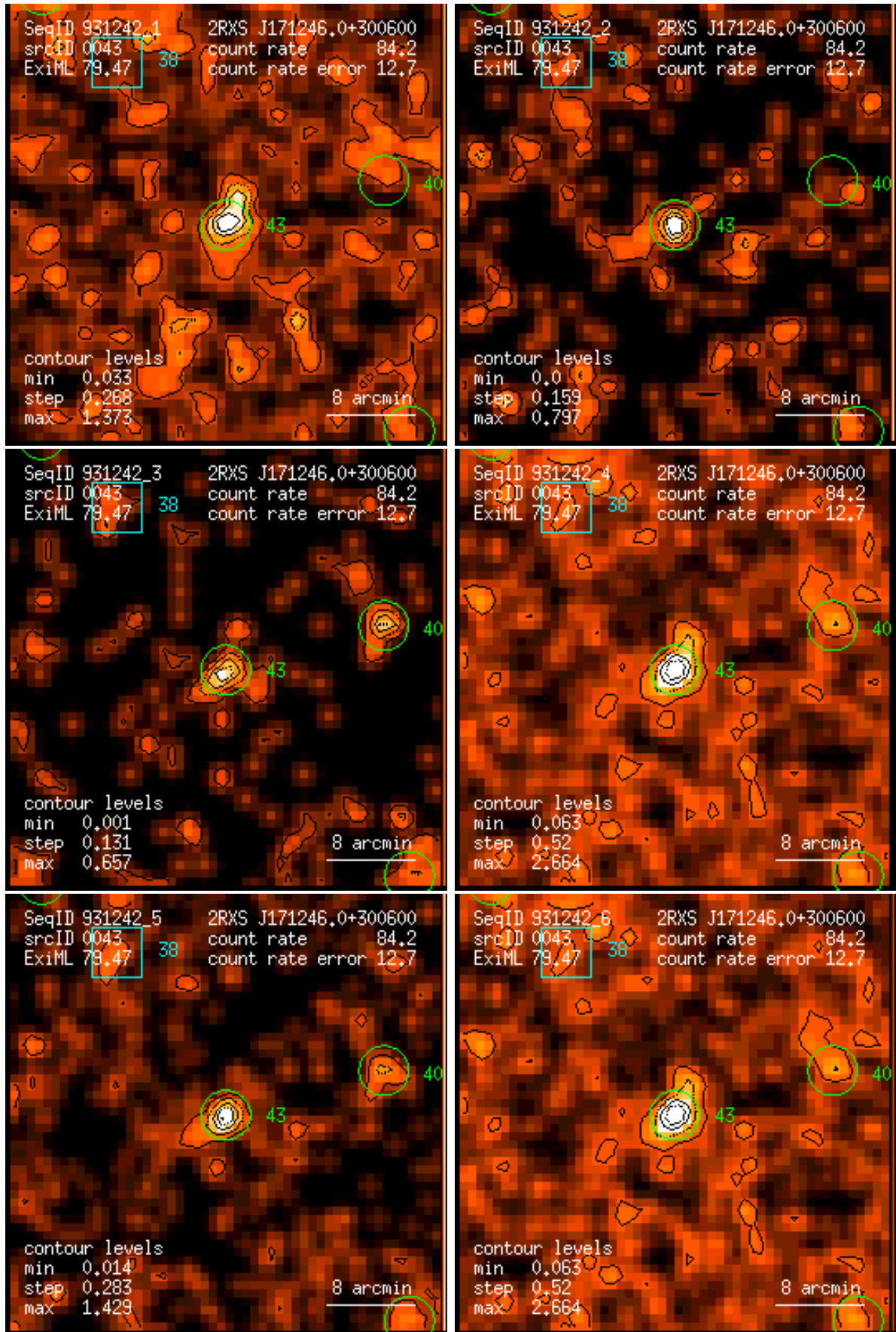
Figure 43: RASS 931242: detection 0043: band rate images, Gaussian filter: (1) PSPC channels 11 – 41, (2) 52 – 90, (3) 91 – 201, (4) 11 – 235, (5) 52 – 201, (6) 11 – 201. Broad band rates in counts/ks. Band rate contour levels in counts/ks/arcmin 2 .
