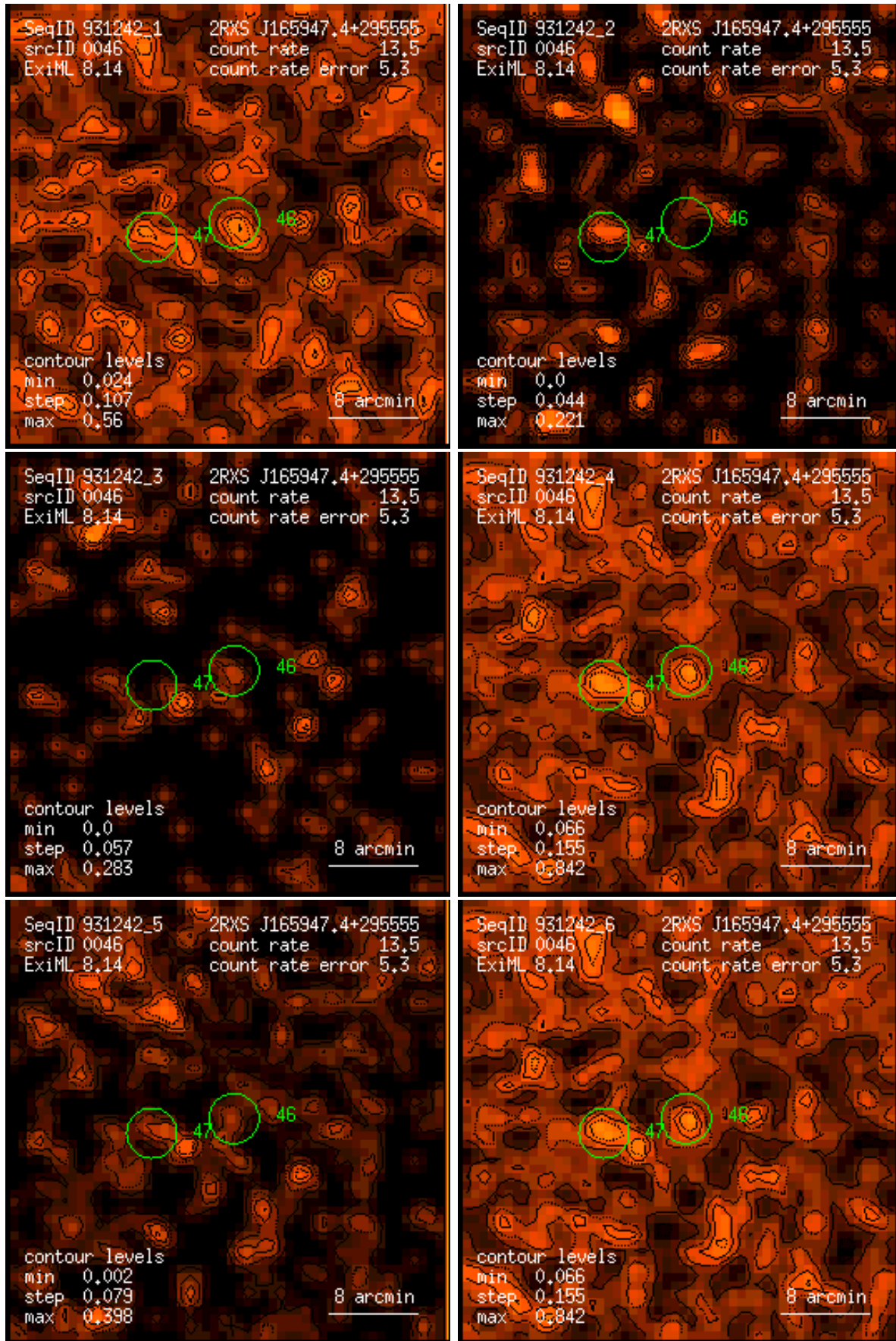
Figure 46: RASS 931242: detection 0046: band rate images, Gaussian filter: (1) PSPC channels 11 – 41, (2) 52 – 90, (3) 91 – 201, (4) 11 – 235, (5) 52 – 201, (6) 11 – 201. Broad band rates in counts/ks. Band rate contour levels in counts/ks/arcmin 2 .
