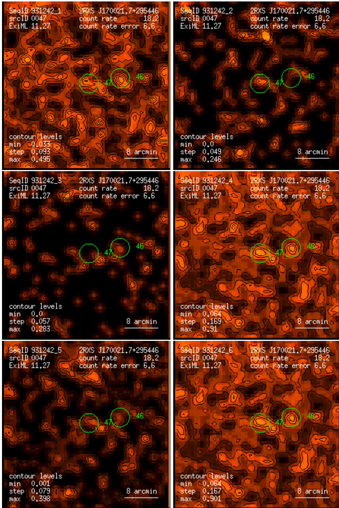
Figure 47: RASS 931242: detection 0047: band rate images, Gaussian filter: (1) PSPC channels 11 – 41, (2) 52 – 90, (3) 91 – 201, (4) 11 – 235, (5) 52 – 201, (6) 11 – 201. Broad band rates in counts/ks. Band rate contour levels in counts/ks/arcmin 2 .
