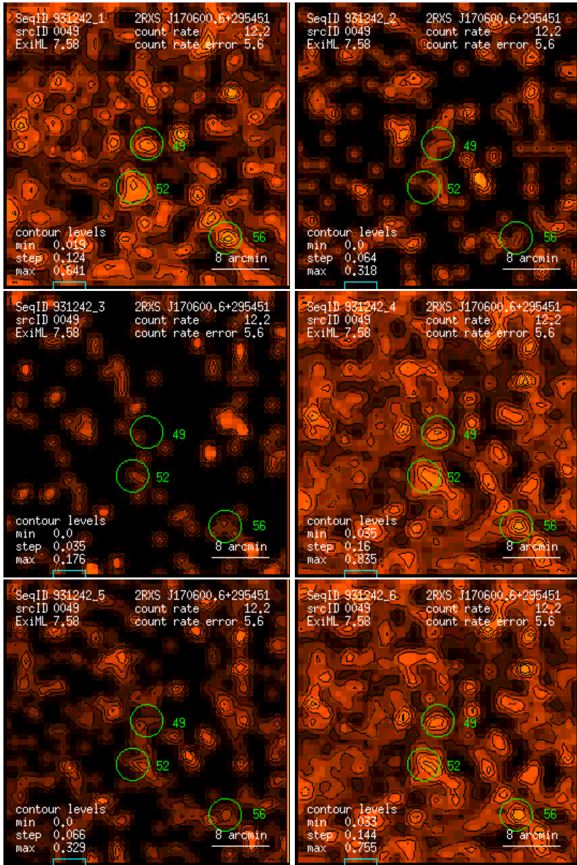
Figure 49: RASS 931242: detection 0049: band rate images, Gaussian filter: (1) PSPC channels 11 – 41, (2) 52 – 90, (3) 91 – 201, (4) 11 – 235, (5) 52 – 201, (6) 11 – 201. Broad band rates in counts/ks. Band rate contour levels in counts/ks/arcmin 2 .
