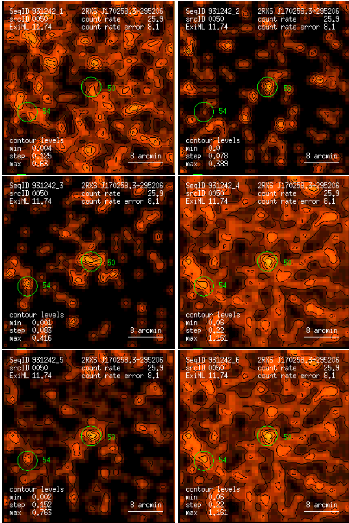
Figure 50: RASS 931242: detection 0050: band rate images, Gaussian filter: (1) PSPC channels 11 – 41, (2) 52 – 90, (3) 91 – 201, (4) 11 – 235, (5) 52 – 201, (6) 11 – 201. Broad band rates in counts/ks. Band rate contour levels in counts/ks/arcmin 2 .
