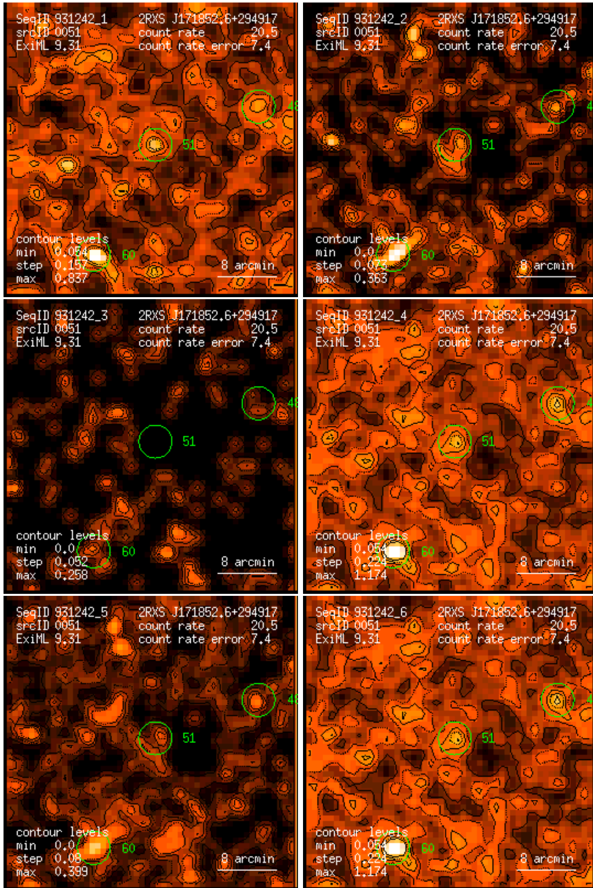
Figure 51: RASS 931242: detection 0051: band rate images, Gaussian filter: (1) PSPC channels 11 – 41, (2) 52 – 90, (3) 91 – 201, (4) 11 – 235, (5) 52 – 201, (6) 11 – 201. Broad band rates in counts/ks. Band rate contour levels in counts/ks/arcmin 2 .
