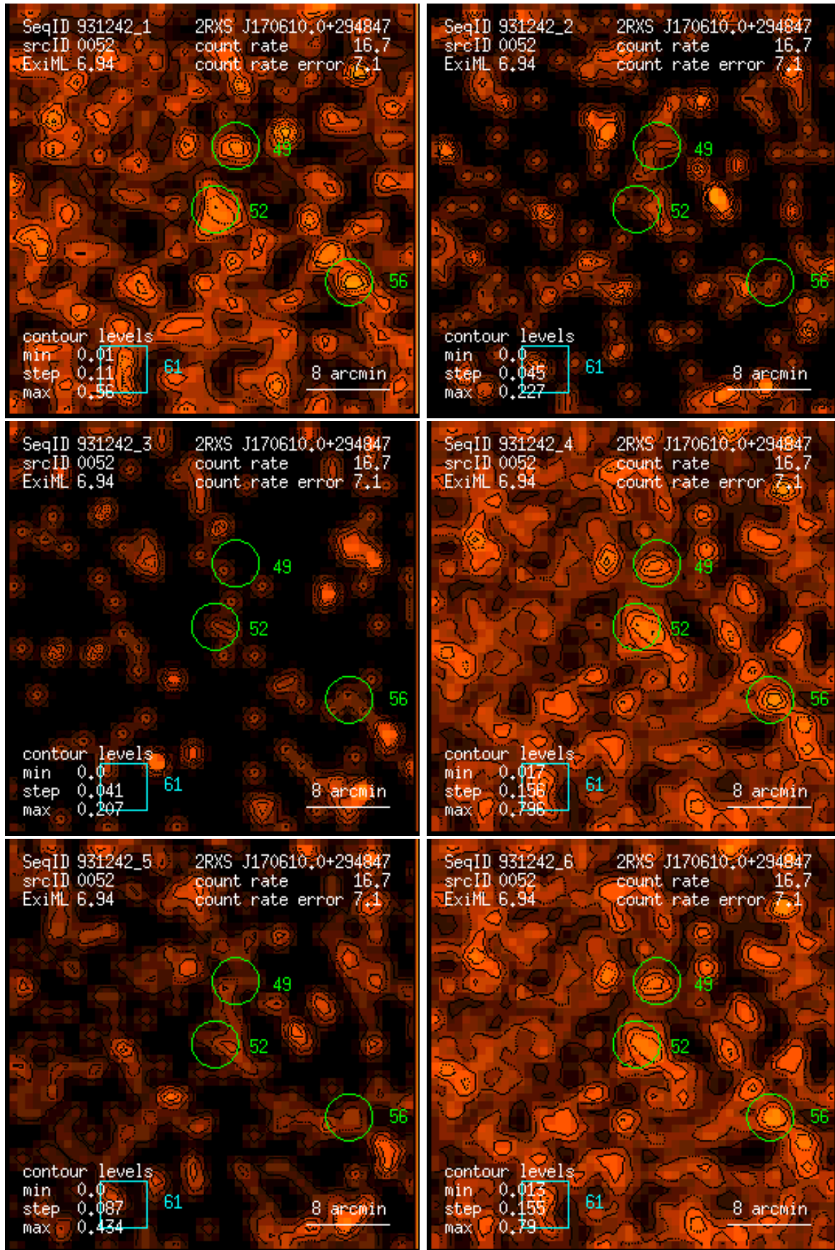
Figure 52: RASS 931242: detection 0052: band rate images, Gaussian filter: (1) PSPC channels 11 – 41, (2) 52 – 90, (3) 91 – 201, (4) 11 – 235, (5) 52 – 201, (6) 11 – 201. Broad band rates in counts/ks. Band rate contour levels in counts/ks/arcmin 2 .
