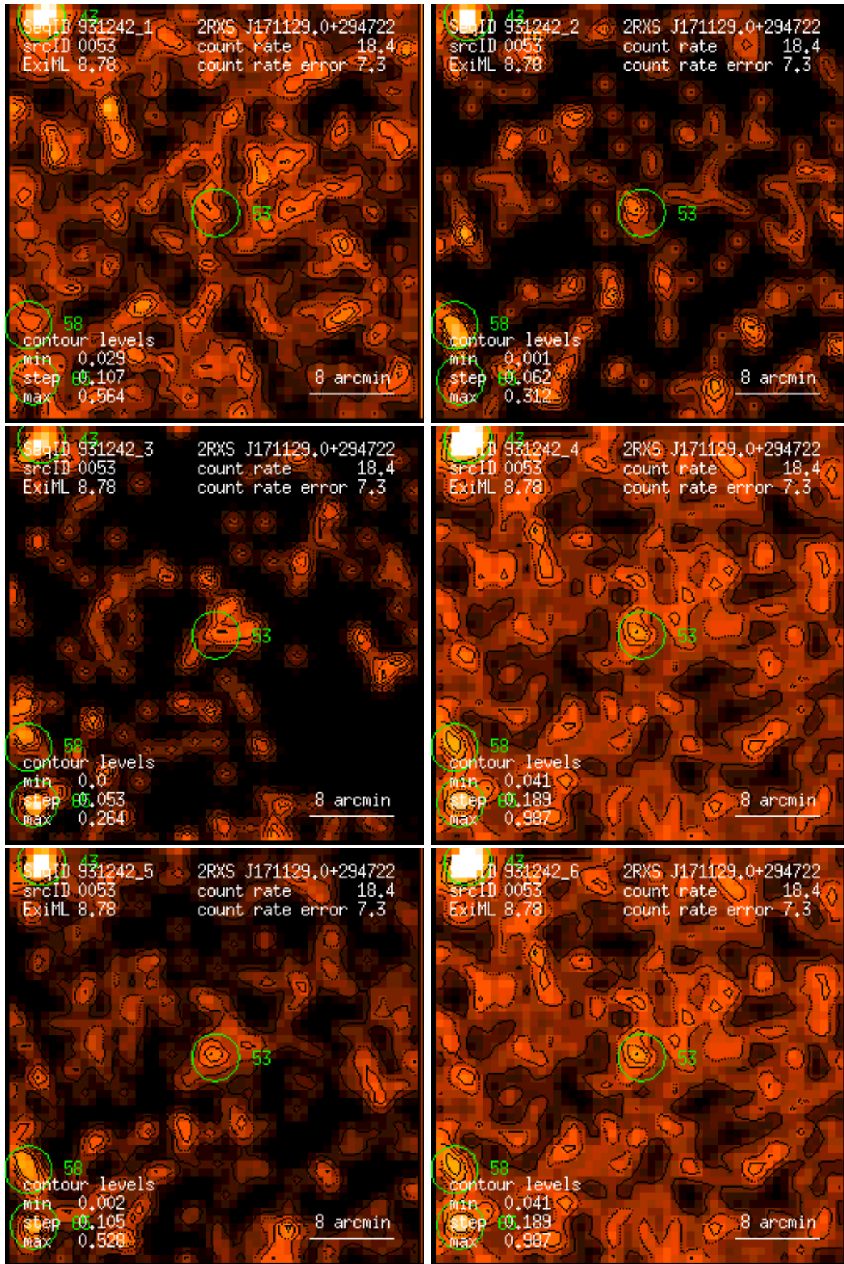
Figure 53: RASS 931242: detection 0053: band rate images, Gaussian filter: (1) PSPC channels 11 – 41, (2) 52 – 90, (3) 91 – 201, (4) 11 – 235, (5) 52 – 201, (6) 11 – 201. Broad band rates in counts/ks. Band rate contour levels in counts/ks/arcmin 2 .
