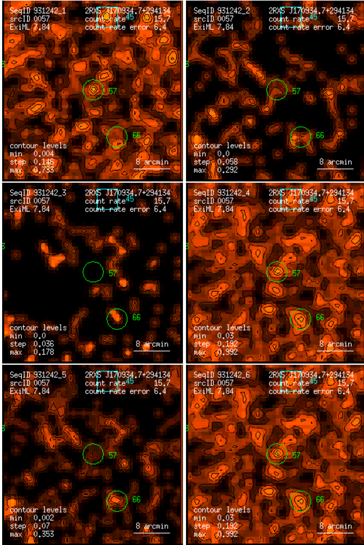
Figure 57: RASS 931242: detection 0057: band rate images, Gaussian filter: (1) PSPC channels 11 – 41, (2) 52 – 90, (3) 91 – 201, (4) 11 – 235, (5) 52 – 201, (6) 11 – 201. Broad band rates in counts/ks. Band rate contour levels in counts/ks/arcmin 2 .
