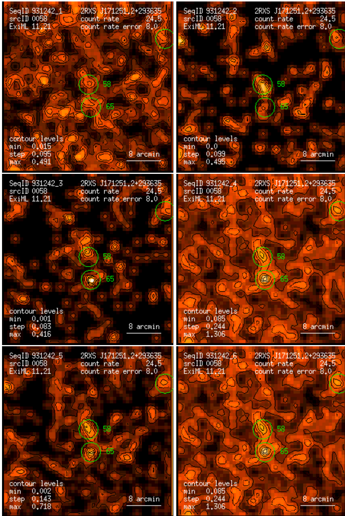
Figure 58: RASS 931242: detection 0058: band rate images, Gaussian filter: (1) PSPC channels 11 – 41, (2) 52 – 90, (3) 91 – 201, (4) 11 – 235, (5) 52 – 201, (6) 11 – 201. Broad band rates in counts/ks. Band rate contour levels in counts/ks/arcmin 2 .
