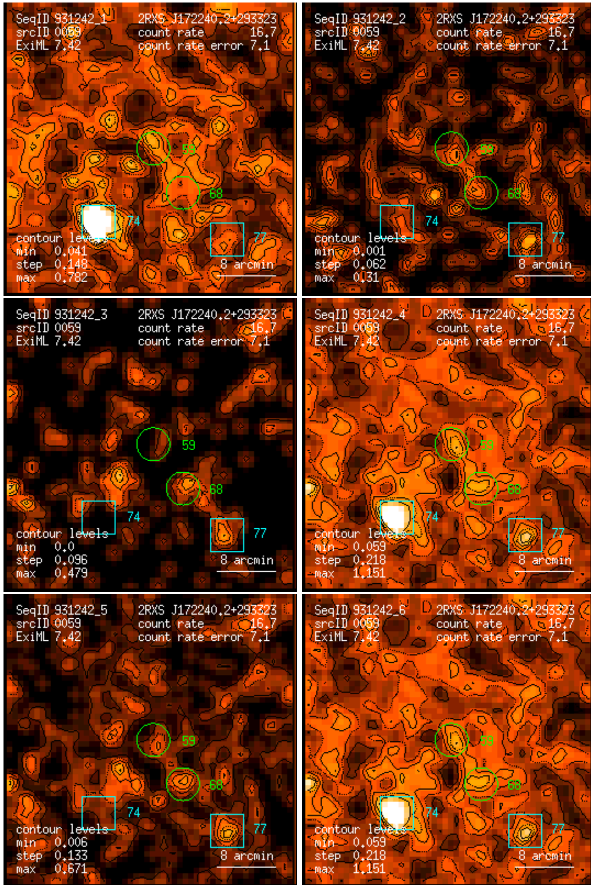
Figure 59: RASS 931242: detection 0059: band rate images, Gaussian filter: (1) PSPC channels 11 – 41, (2) 52 – 90, (3) 91 – 201, (4) 11 – 235, (5) 52 – 201, (6) 11 – 201. Broad band rates in counts/ks. Band rate contour levels in counts/ks/arcmin 2 .
