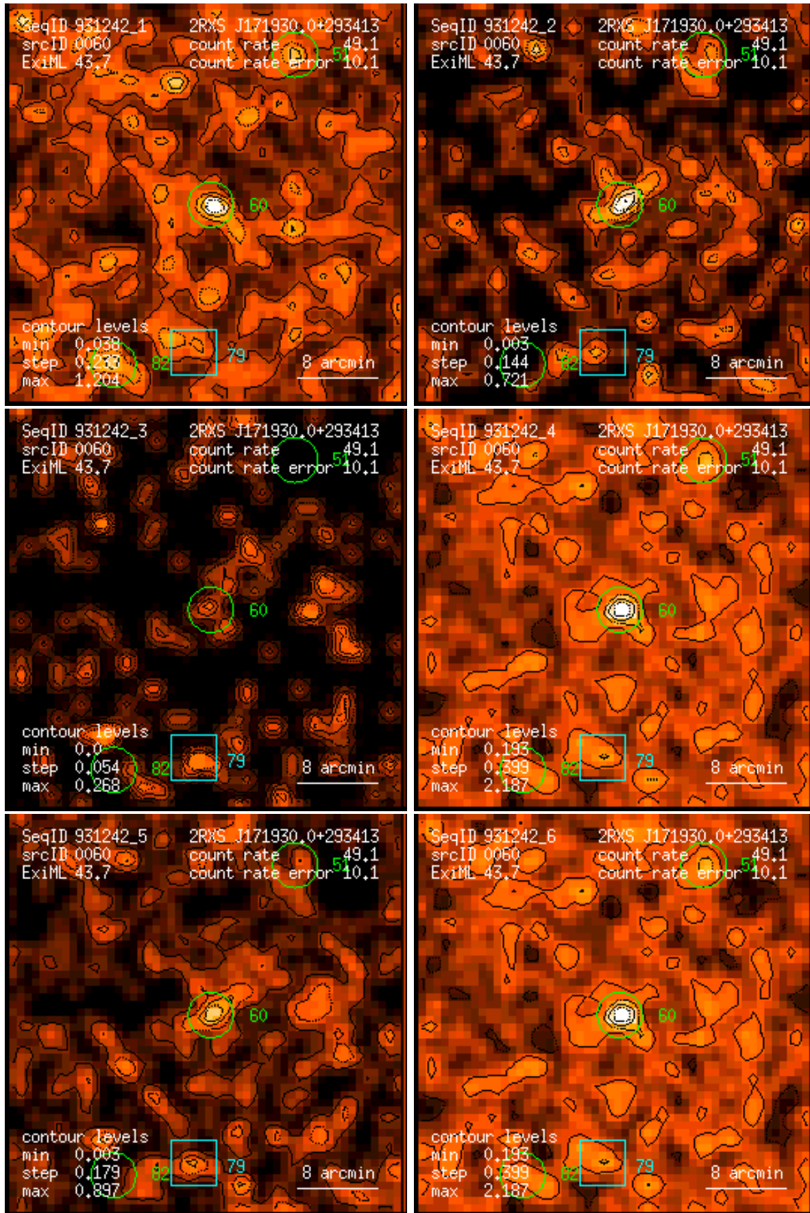
Figure 60: RASS 931242: detection 0060: band rate images, Gaussian filter: (1) PSPC channels 11 – 41, (2) 52 – 90, (3) 91 – 201, (4) 11 – 235, (5) 52 – 201, (6) 11 – 201. Broad band rates in counts/ks. Band rate contour levels in counts/ks/arcmin 2 .
