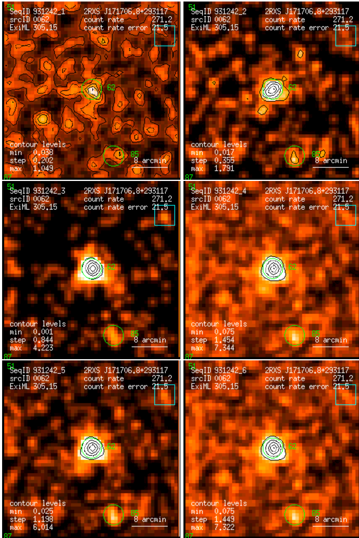
Figure 62: RASS 931242: detection 0062: band rate images, Gaussian filter: (1) PSPC channels 11 – 41, (2) 52 – 90, (3) 91 – 201, (4) 11 – 235, (5) 52 – 201, (6) 11 – 201. Broad band rates in counts/ks. Band rate contour levels in counts/ks/arcmin 2 .
