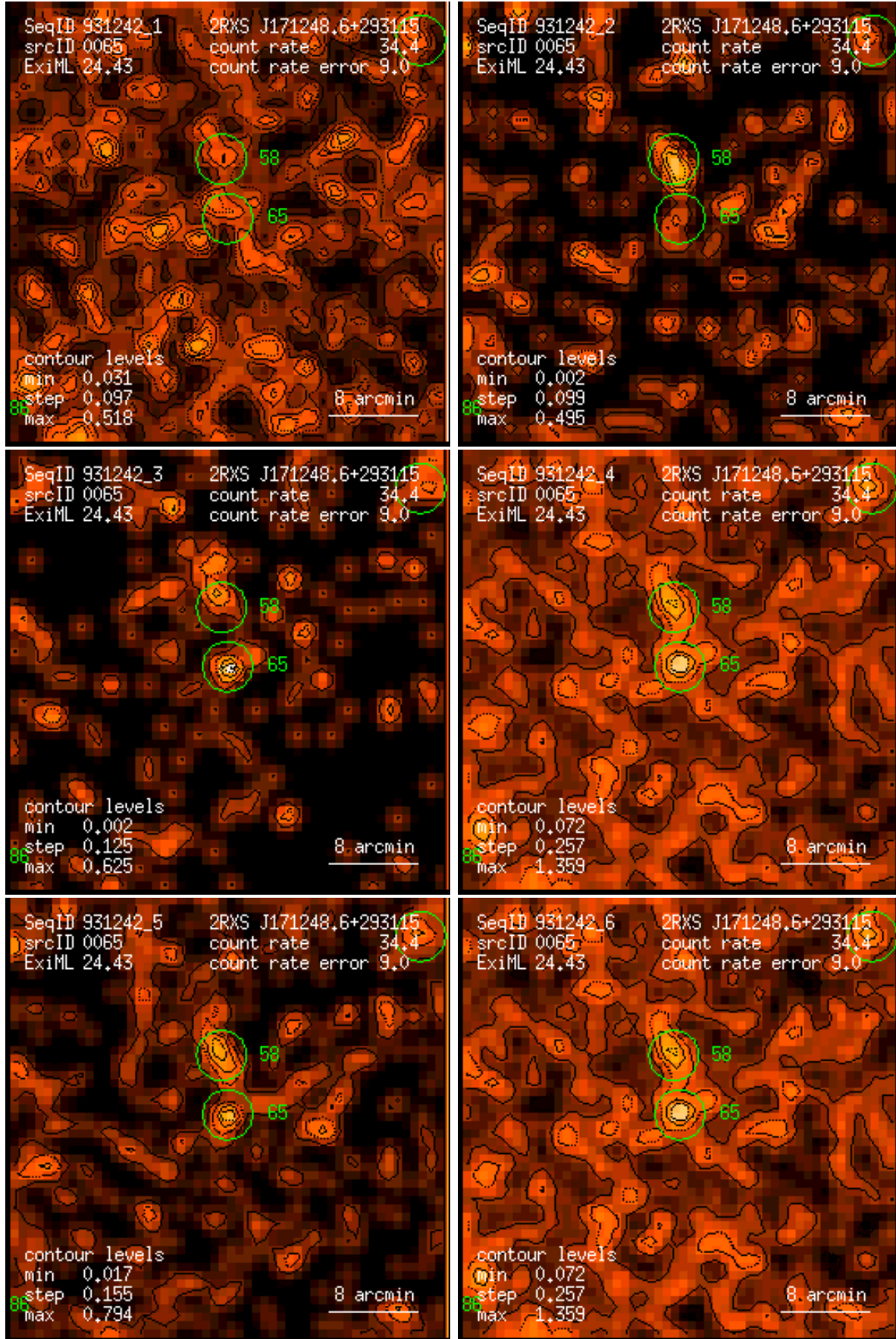
Figure 65: RASS 931242: detection 0065: band rate images, Gaussian filter: (1) PSPC channels 11 – 41, (2) 52 – 90, (3) 91 – 201, (4) 11 – 235, (5) 52 – 201, (6) 11 – 201. Broad band rates in counts/ks. Band rate contour levels in counts/ks/arcmin 2 .
