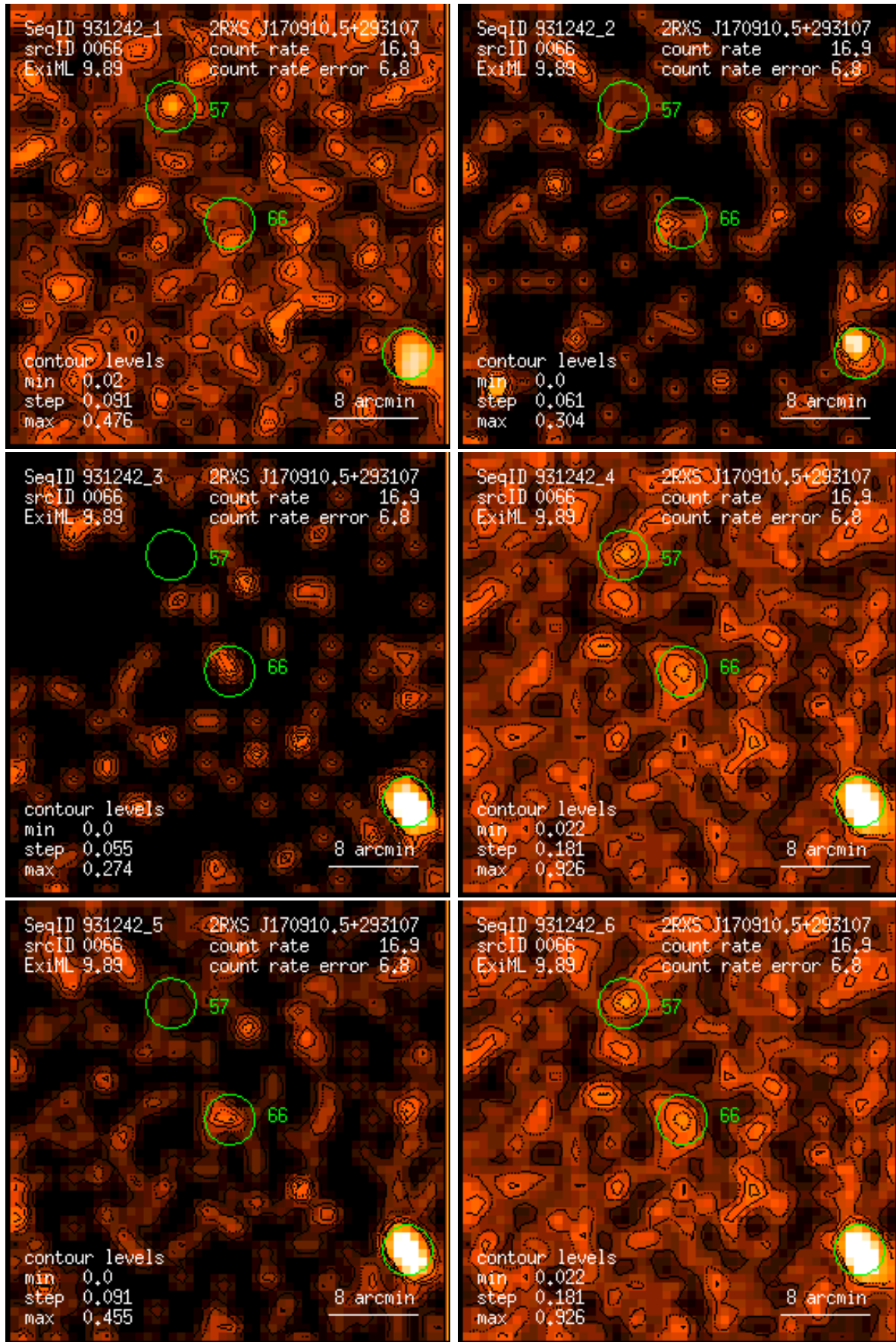
Figure 66: RASS 931242: detection 0066: band rate images, Gaussian filter: (1) PSPC channels 11 – 41, (2) 52 – 90, (3) 91 – 201, (4) 11 – 235, (5) 52 – 201, (6) 11 – 201. Broad band rates in counts/ks. Band rate contour levels in counts/ks/arcmin 2 .
